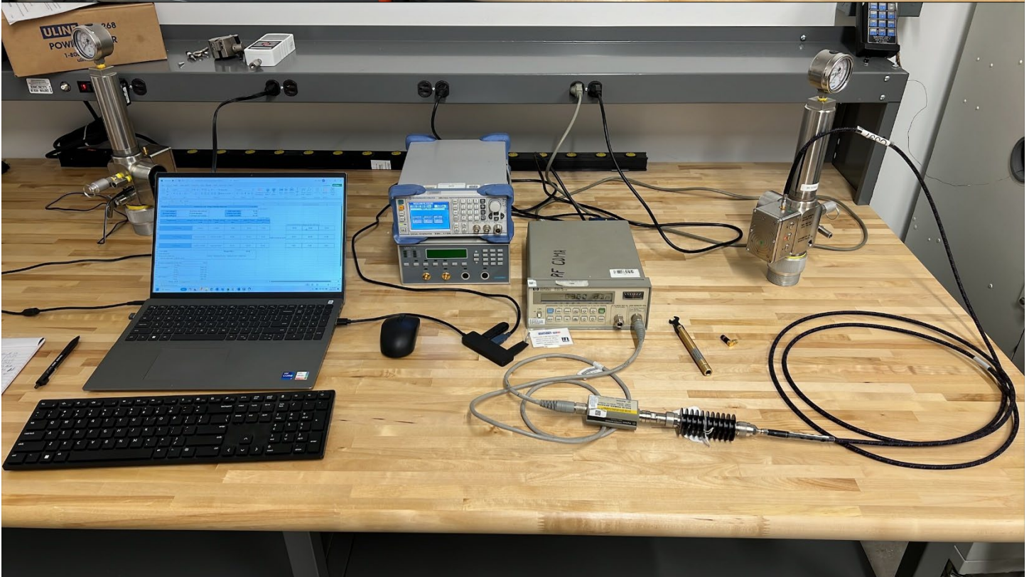
Power, Bandwidth, PSD, Conducted Spurious, Band Edge
