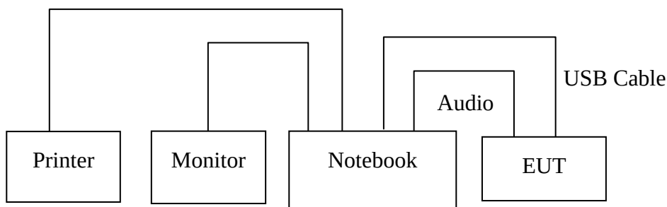
Fig. 2-2 Configuration of Tested System (Audio-in Mode)
