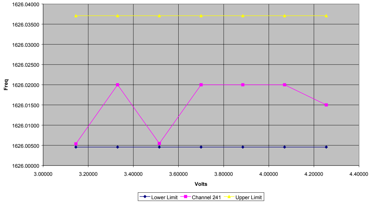
Channel 241 Frequency Stability - Voltage
