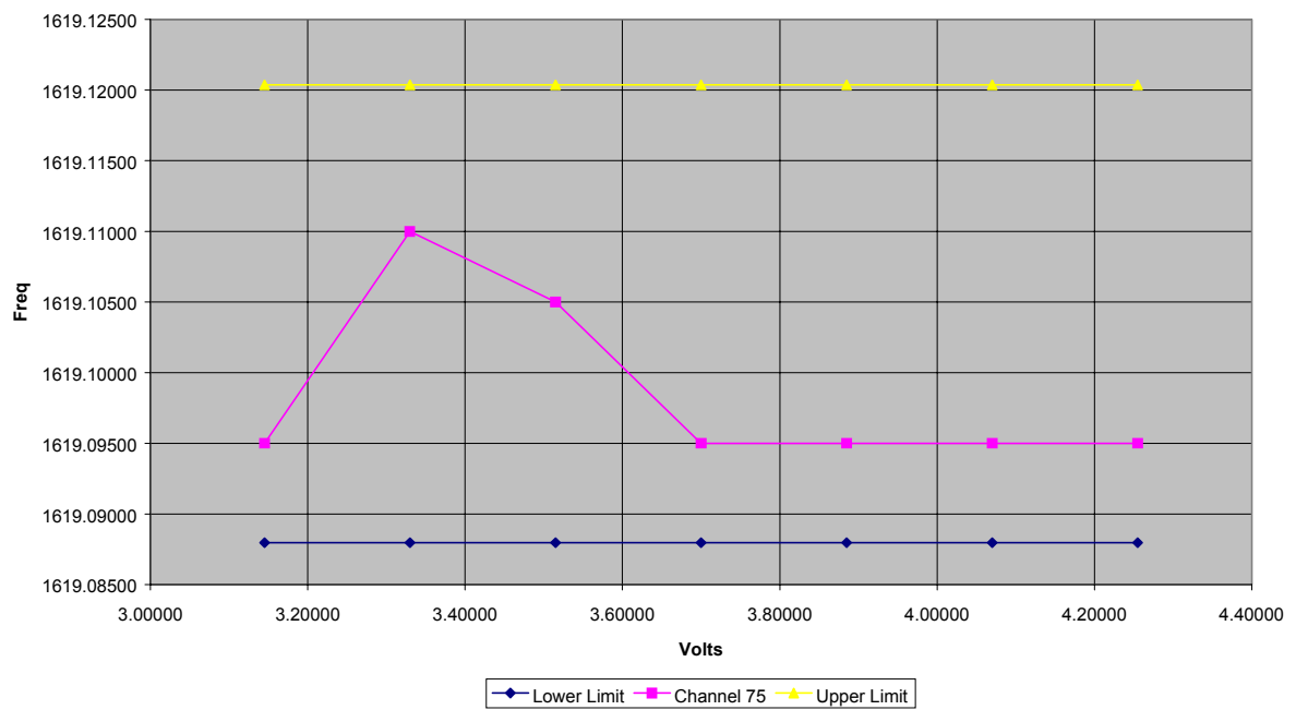
Channel 75 Frequency Stability - Voltage
