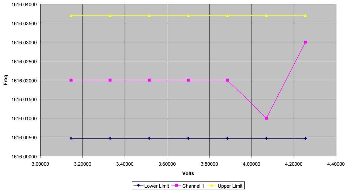
Channel 1 Frequency Stability - Voltage
