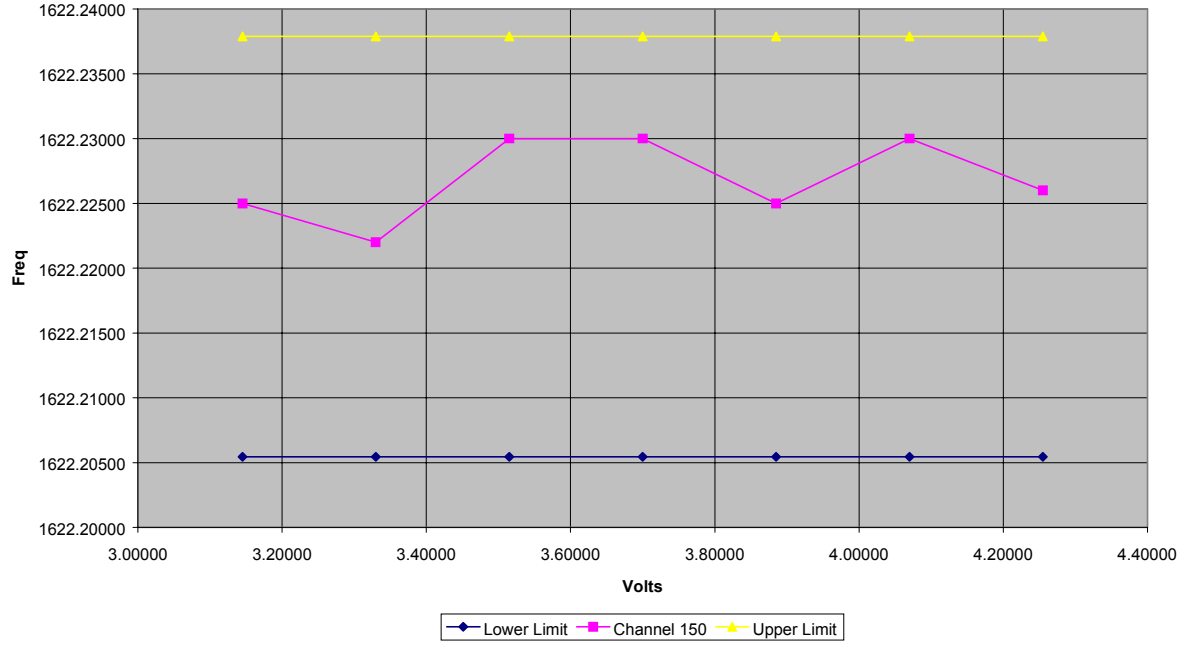
Channel 150 Frequency Stability - Voltage
