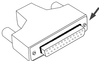
Figure 6: Place a bead of Silicone RTV material along this area all around the connector mating to the 9522A LBT's multi-interface connector.
