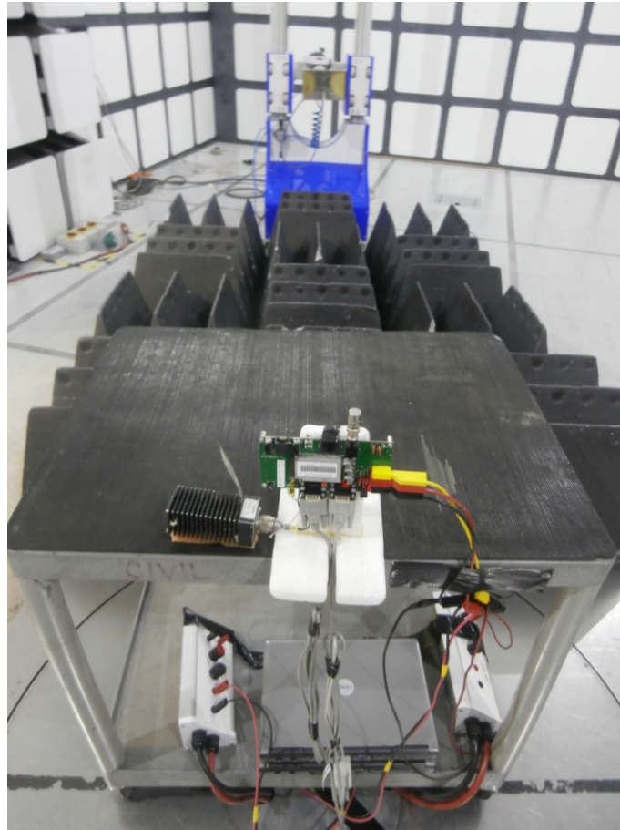
Radiated Emissions 1 GHz to 18 GHz – Upright Orientation
