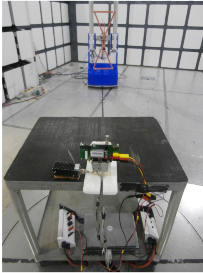
Radiated Emissions 30 MHz to 1 GHz – Upright Orientation
