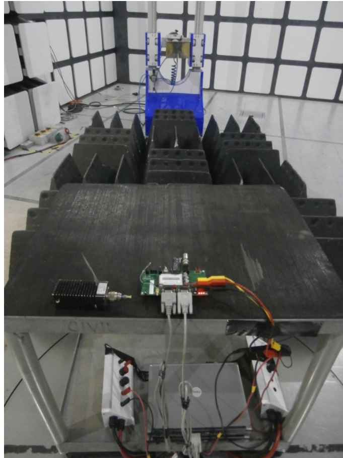
Radiated Emissions 1 GHz to 18 GHz – Flat Orientation
