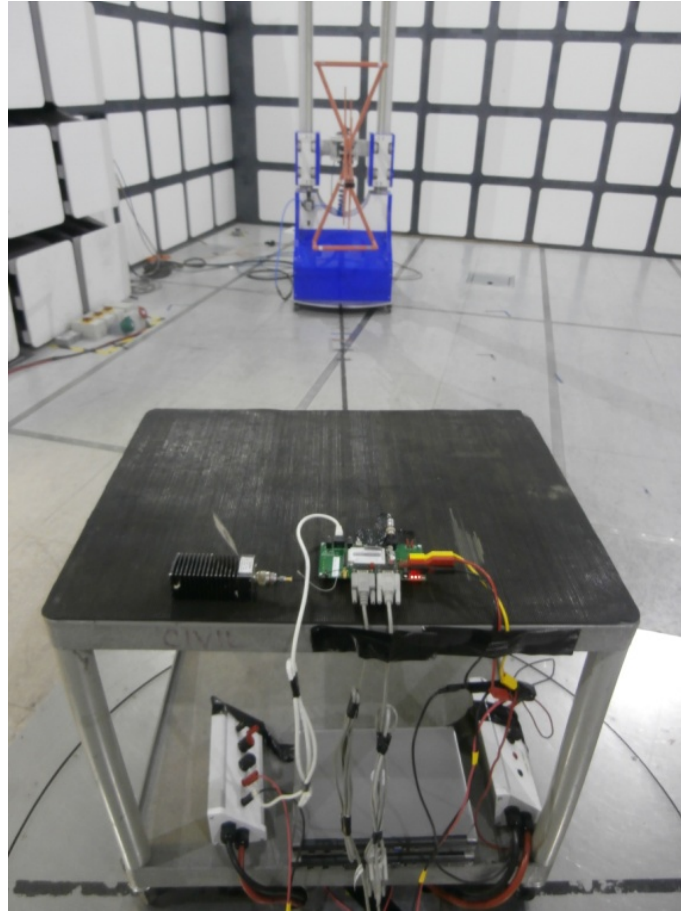
Radiated Emissions 30 MHz to 1 GHz – Flat Orientation
