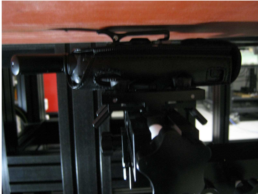
SAR: Body Testing- Belt Holder- Antenna Position 3
