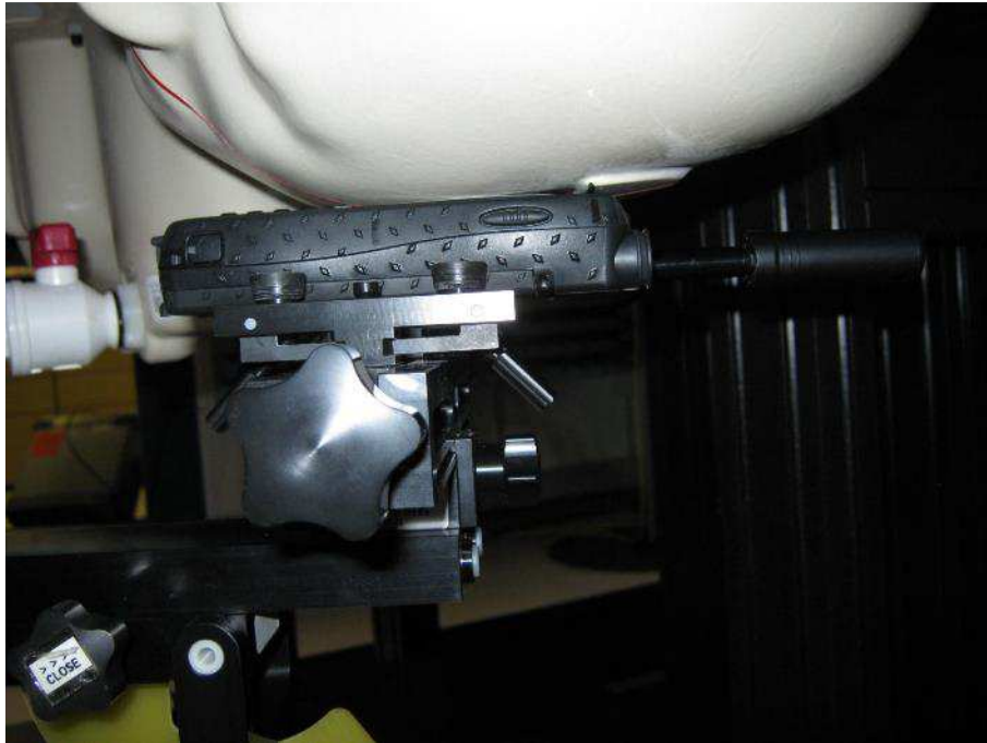
SAR: LH Cheek- Antenna Position 2 (Retracted by 50mm)
