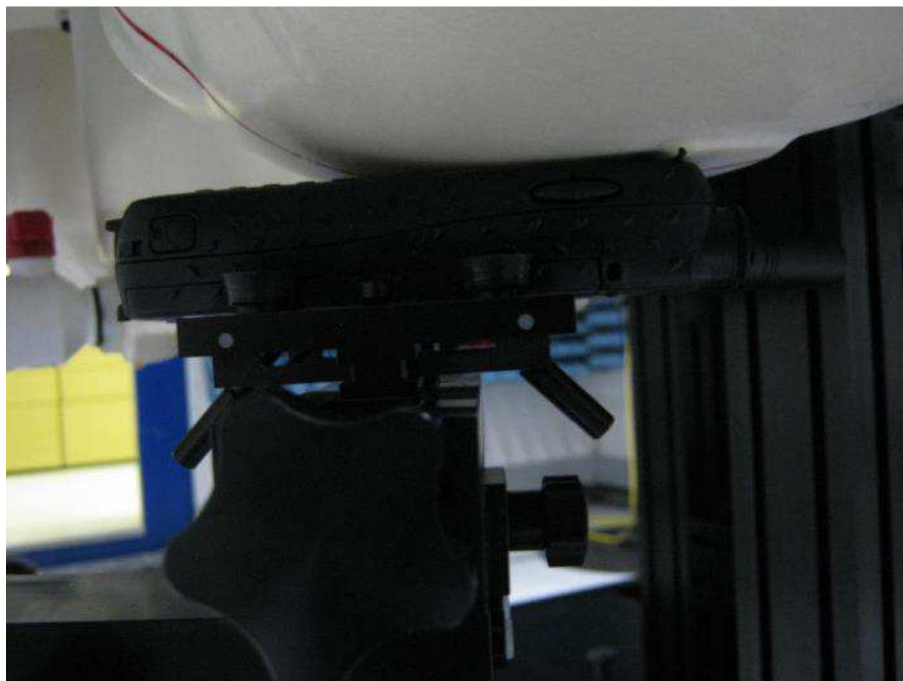
SAR: LH Cheek-Antenna Retracted - Position 1
