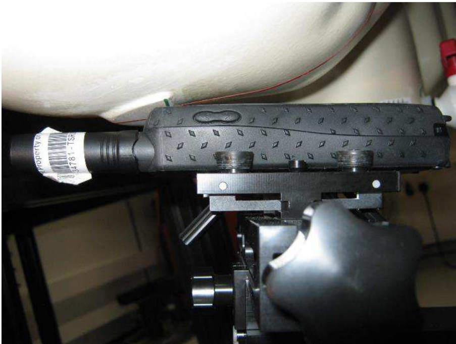
SAR: RH 15° Tilt -Antenna Retracted - Position 2
