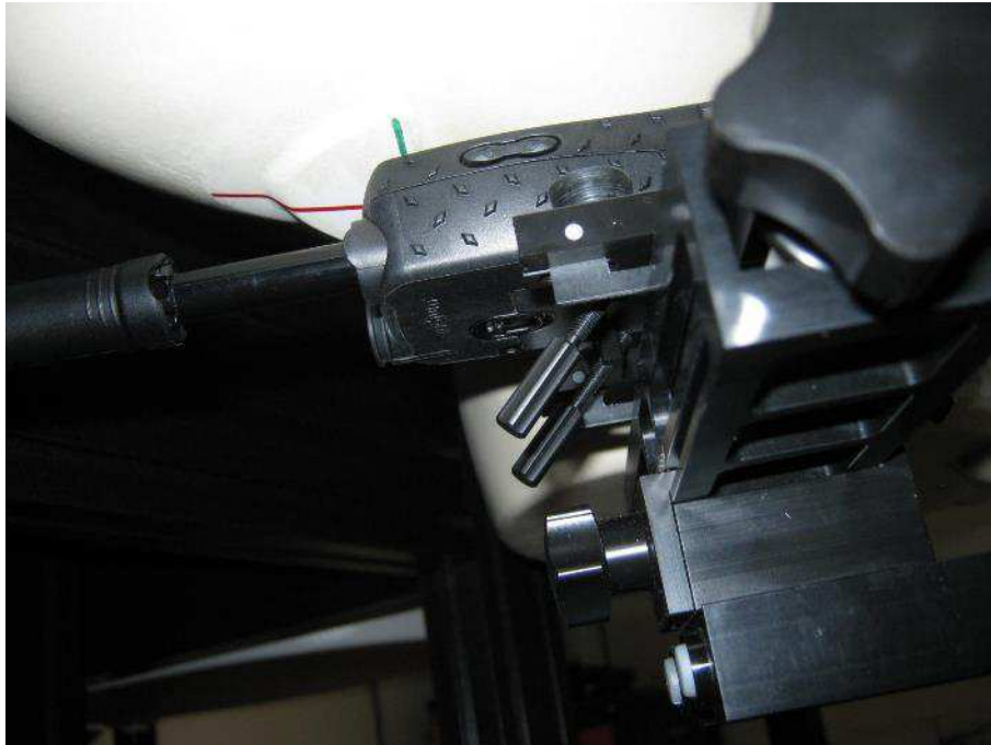
SAR: RH Cheek- Antenna Position 2 (Retracted by 50mm)
