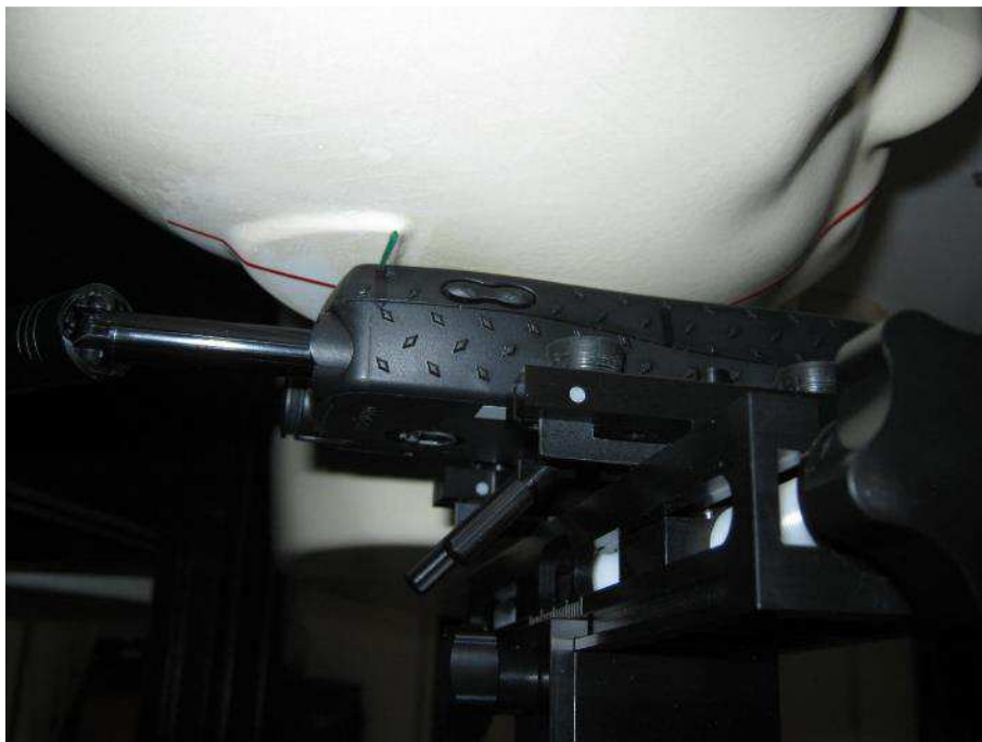
SAR: RH Cheek- Antenna Position 3 (Retracted by 50mm)
