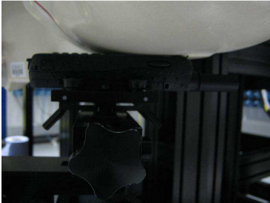
SAR: LH Cheek-Antenna Retracted - Position 2
