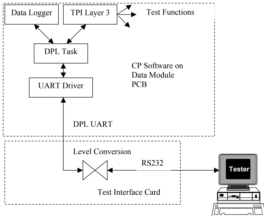
Figure 7: Test Configuration
