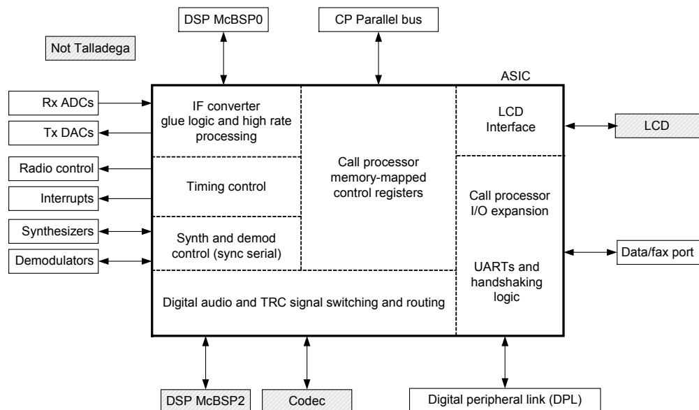
Figure 4: ASIC Logic
