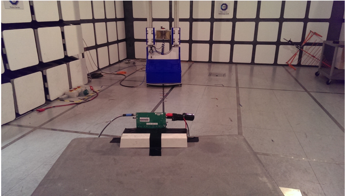
Radiated Emissions 1-17GHz
