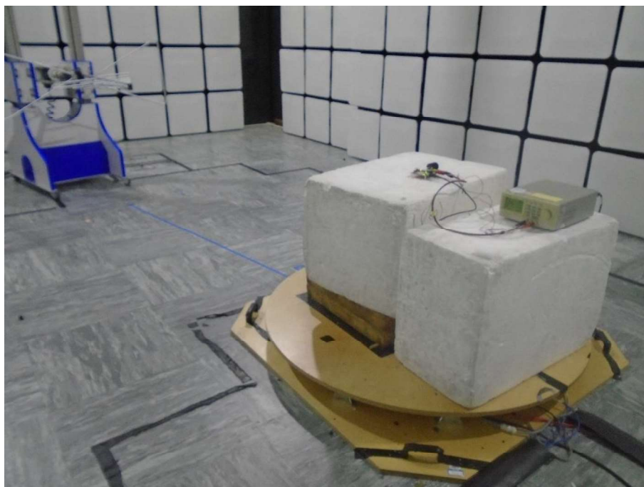
Figure 139 - 30MHz to 1GHz Setup X Plane
