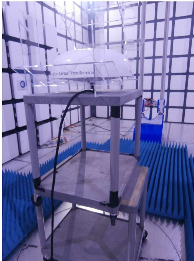
FCC Part 25 Radiated Emissions/EIRP - 1 GHz to 18 GHz – Horizontal
