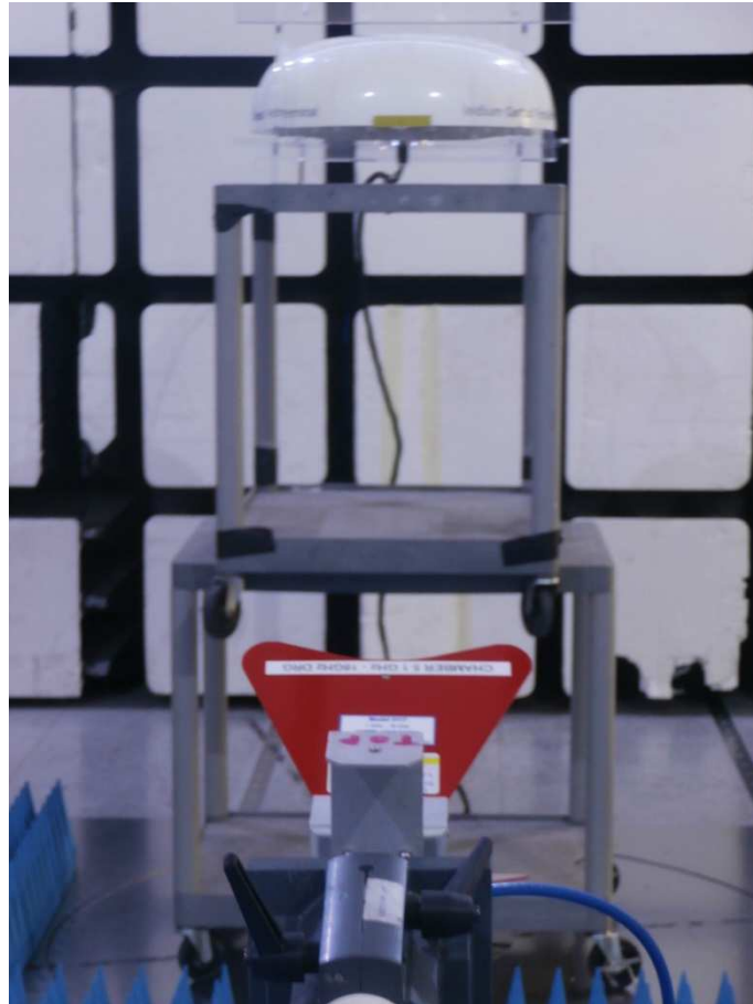
FCC Part 25 Radiated Emissions/EIRP - 1 GHz to 18 GHz – Reference View – Horizontal
