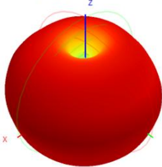
2500.0MHz H+V, Eff: 46.4%
