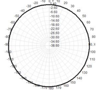
Total(H-XY), Max= 0.67dBi, CirD=0.79
