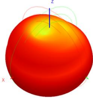
2400.0MHz H+V, Eff: 59.9%
