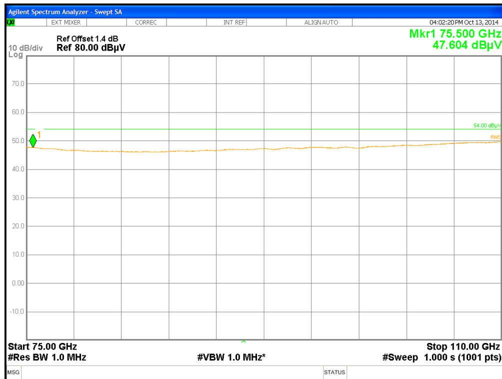
Plot 21: 75 GHz – 110 GHz, special test mode, flow/mid/high
