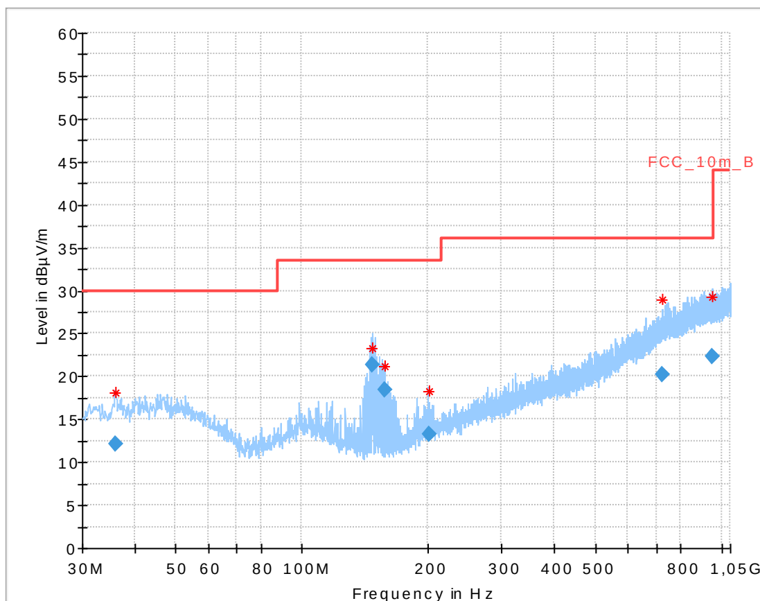
Plot 4: 30 MHz – 1000 MHz, special test mode, frequency sweep stopped at f_{\text{high}}
