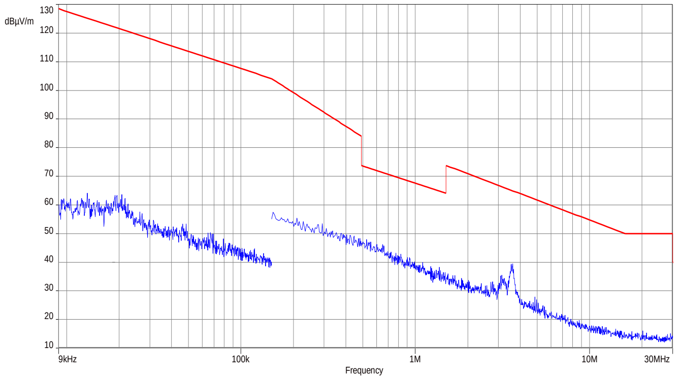
Plot 2: 9 kHz – 30 MHz, special test mode, f_{low}/f_{mid}/f_{high} , PA/FF Bus
