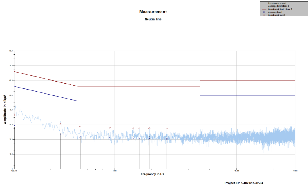
Plot 14: Neutral, HART Bus
