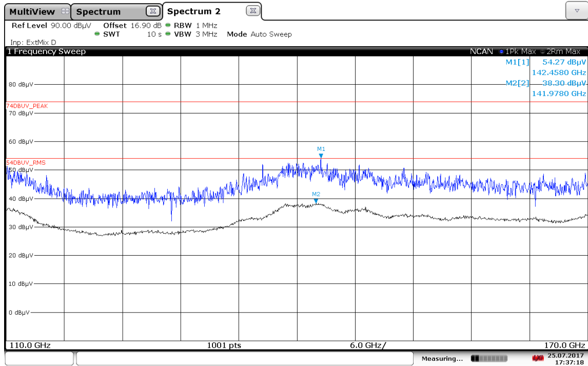
Plot 11: 110 GHz – 170 GHz, PEAK/RMS-measurement, special test mode, f_{\text{low}}/f_{\text{mid}}/f_{\text{high}}
