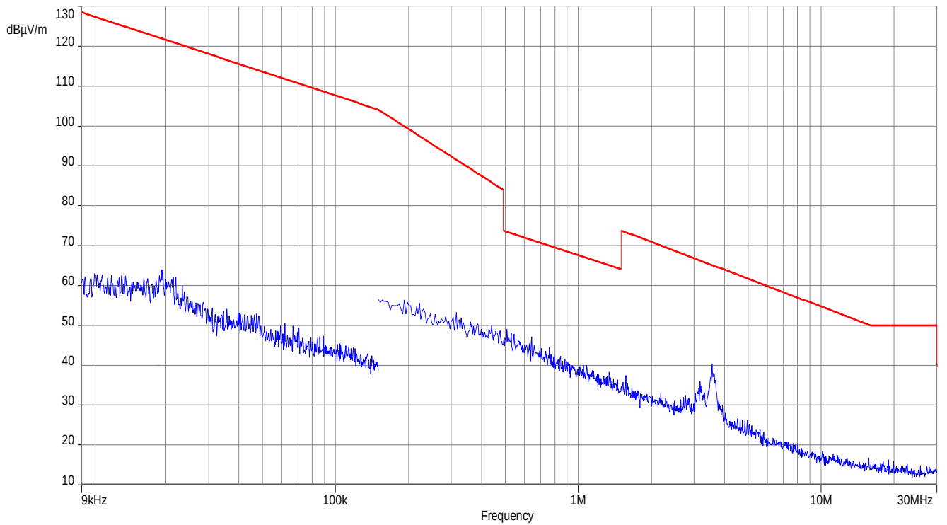
Plot 1: 9 kHz – 30 MHz, special test mode, f_{low}/f_{mid}/f_{high} , HART Bus
