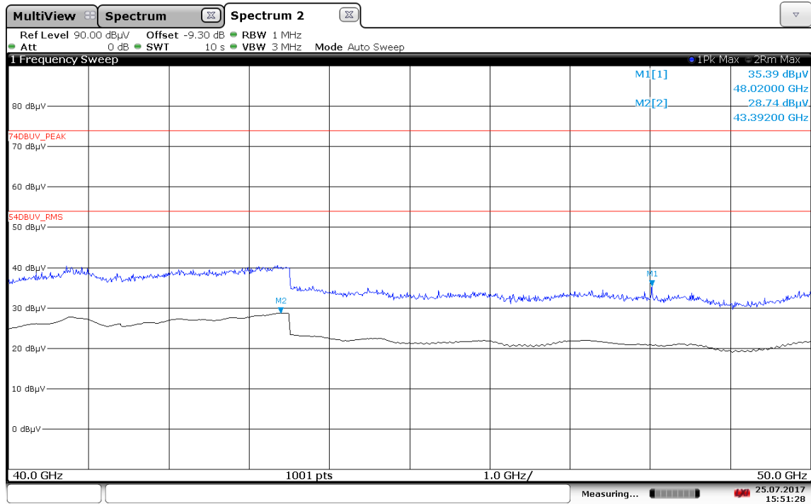
Plot 8: 40 GHz – 50 GHz, PEAK/RMS-measurement, special test mode, f_{low}/f_{mid}/f_{high}
