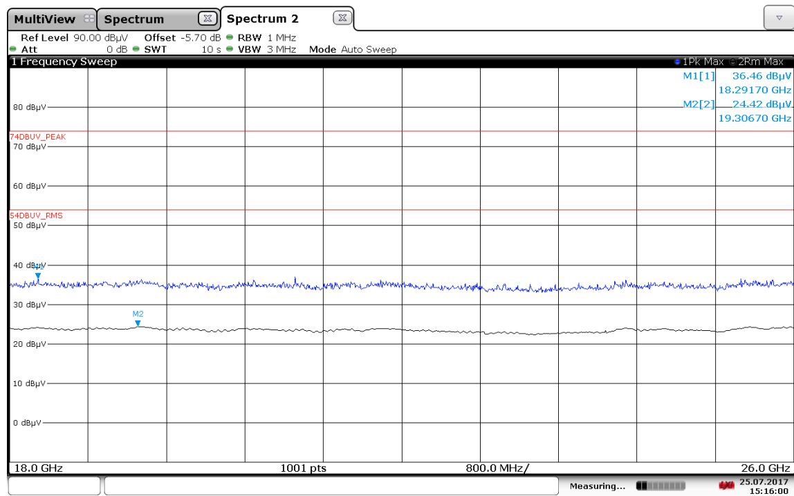
Plot 6: 18 GHz – 26 GHz, PEAK/RMS-measurement, special test mode, f_{low}/f_{mid}/f_{high}
