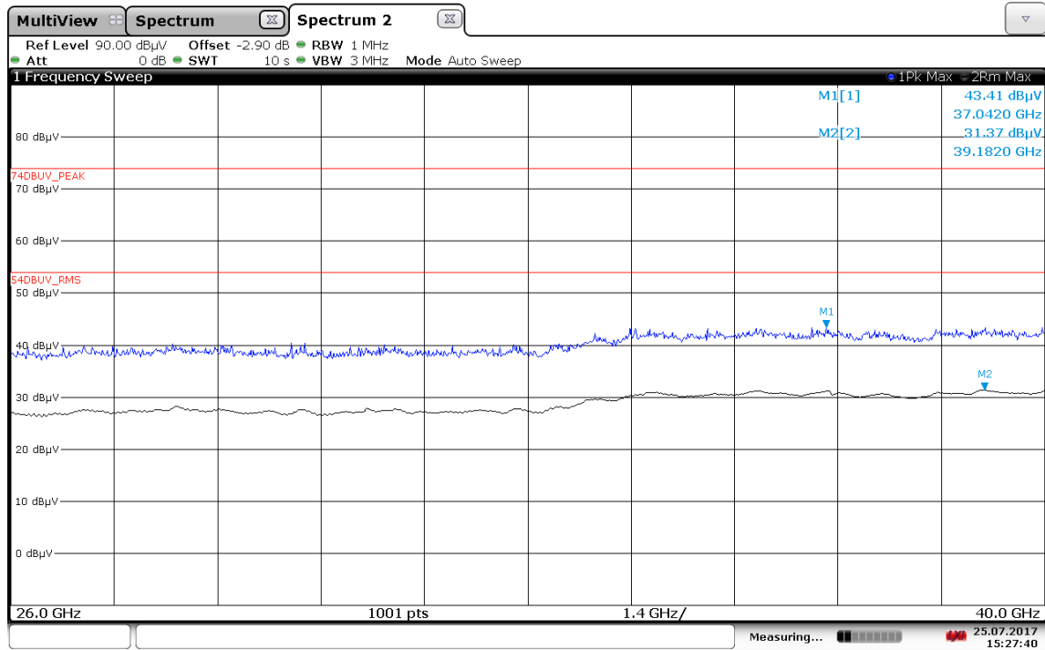
Plot 7: 26 GHz – 40 GHz, PEAK/RMS-measurement, special test mode, f_{low}/f_{mid}/f_{high}
