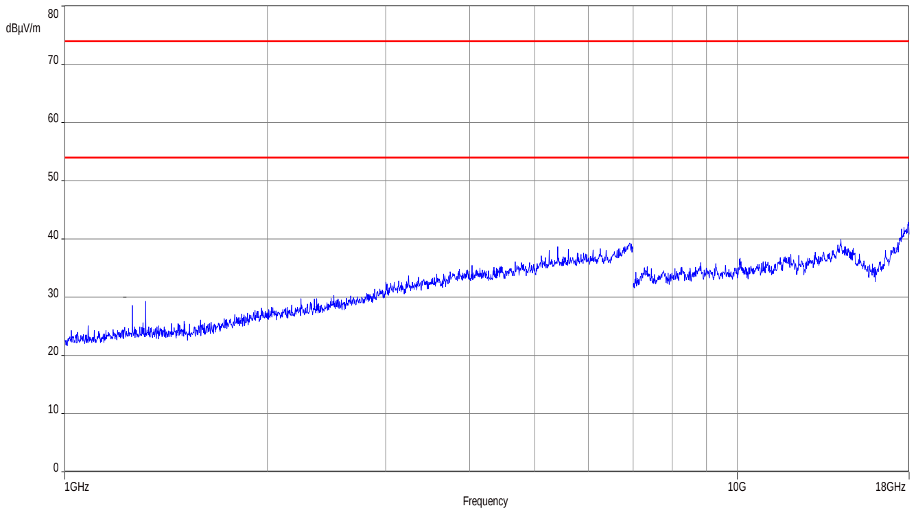
Plot 5: 1 GHz – 18 GHz, PEAK measurement, special test mode, f_{low}/f_{mid}/f_{high}
