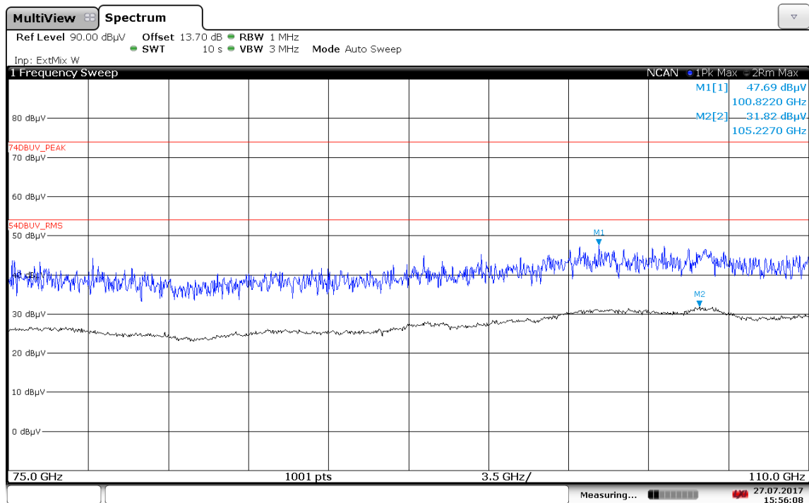
Plot 10: 75 GHz – 110 GHz, PEAK/RMS-measurement, special test mode, f_{\text{low}}/f_{\text{mid}}/f_{\text{high}}
