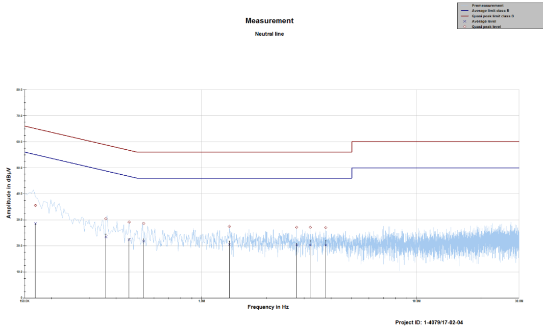
Plot 16: Neutral, PA/FF Bus
