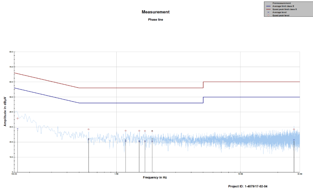
Plot 15: Phase, PA/FF Bus
