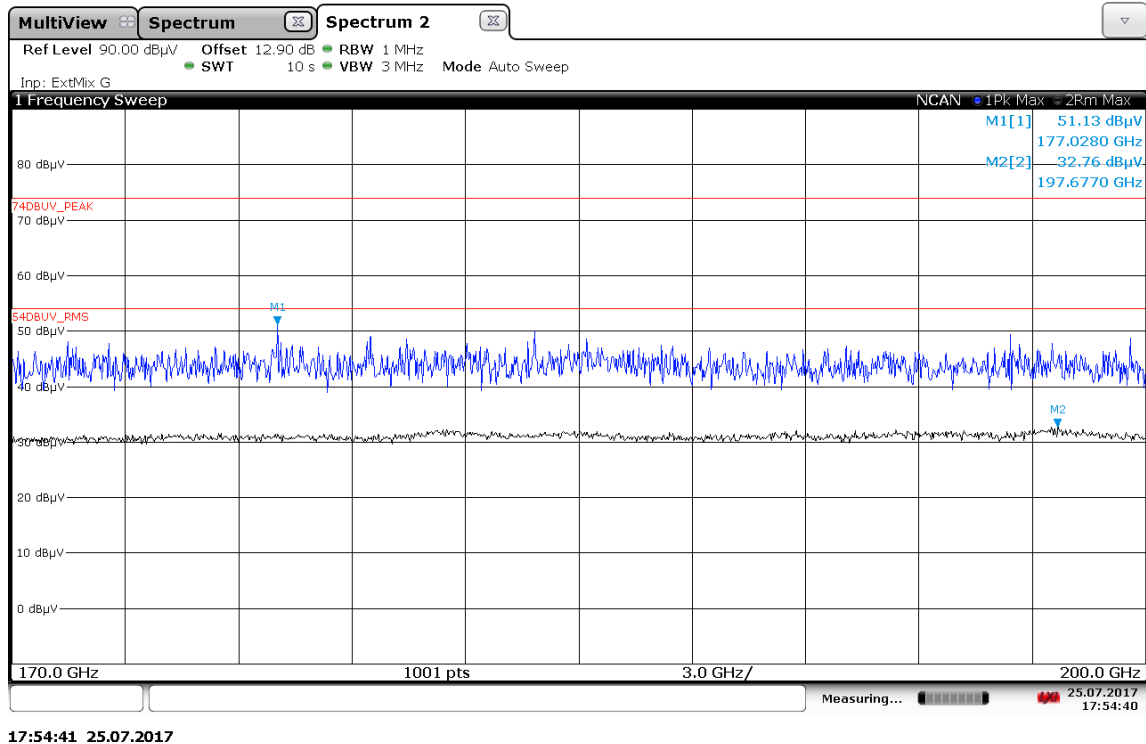
Plot 12: 170 GHz – 200 GHz, PEAK/RMS-measurement, special test mode, f_{\text{low}}/f_{\text{mid}}/f_{\text{high}}
