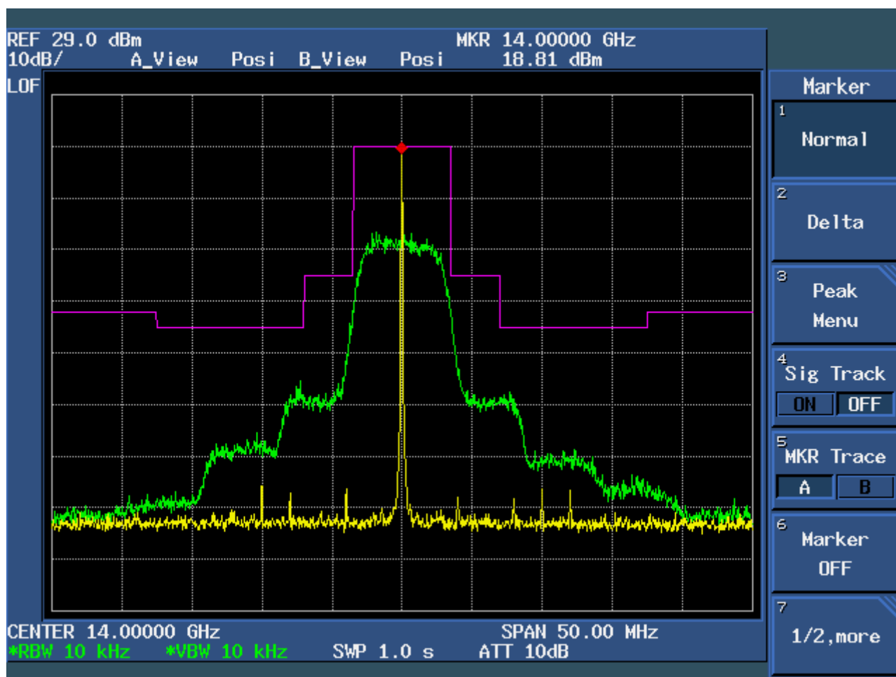
Plot #10: Lowest Channel: 14 GHz, Emission Mask
