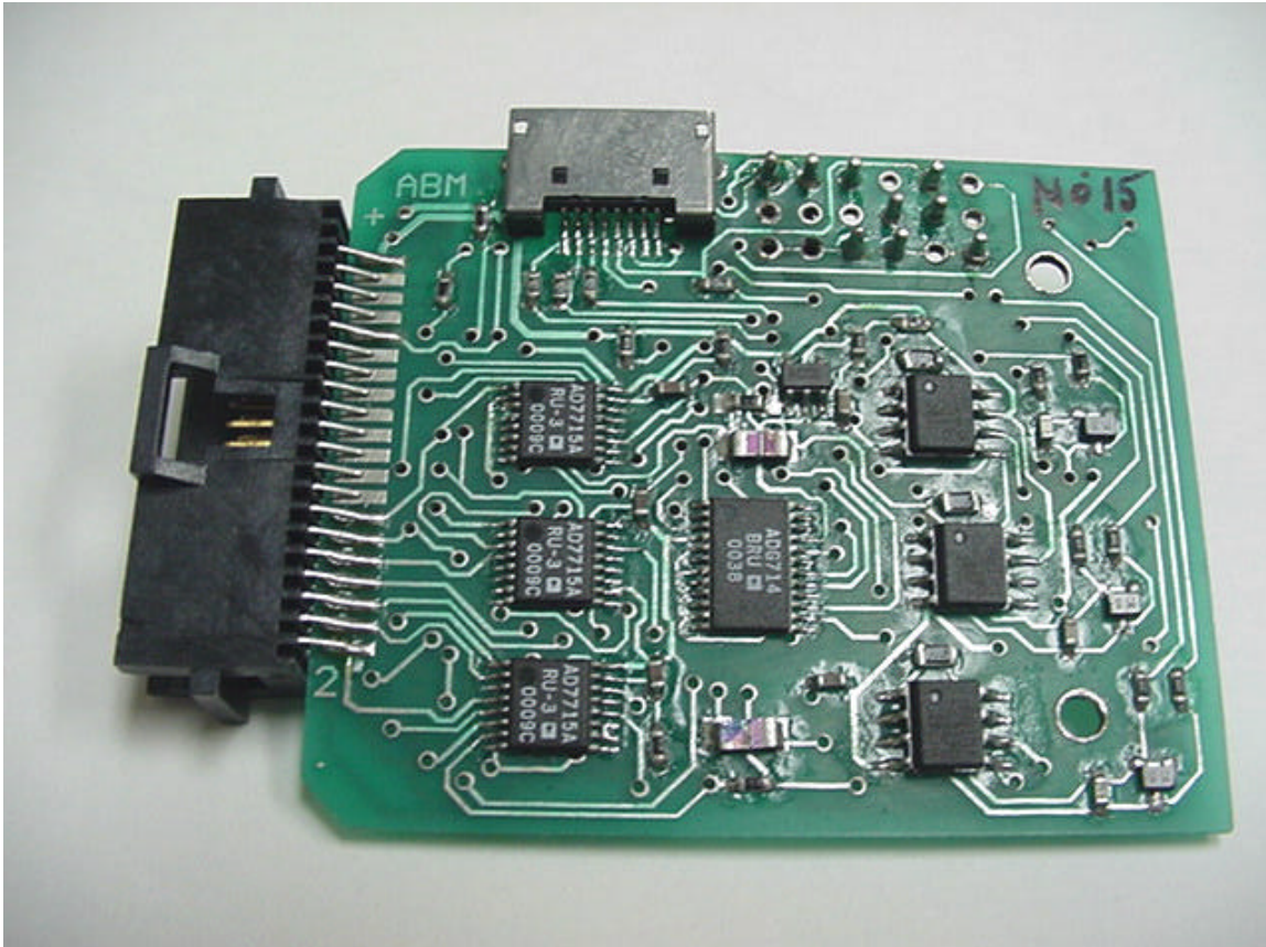
Head Unit 6Channel Board – Top View
