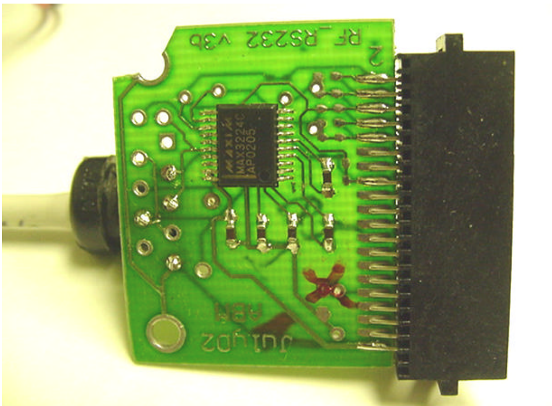
Host Unit Serial Board – Bottom View
