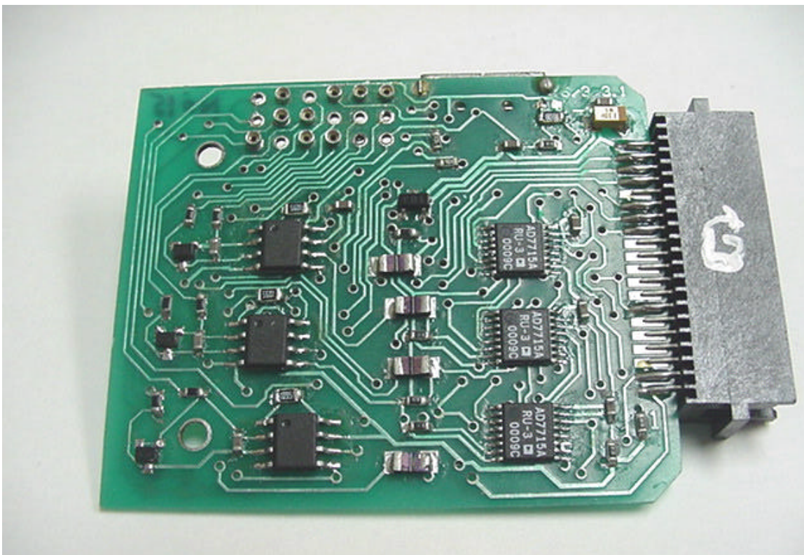
Head Unit 6Channel Board – Bottom View
