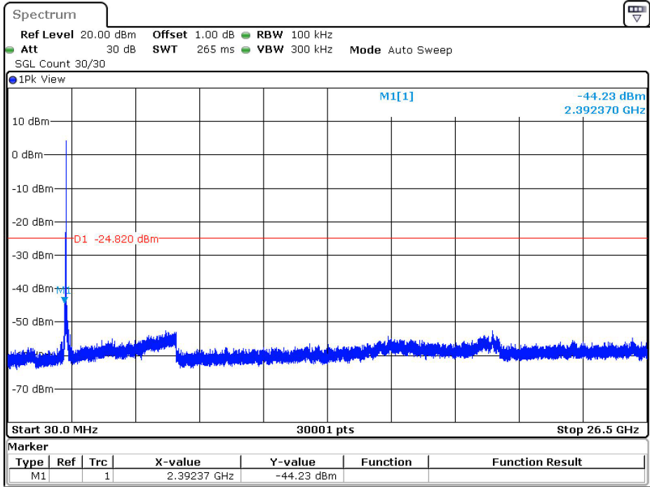
Channel 06 (2437MHz)
