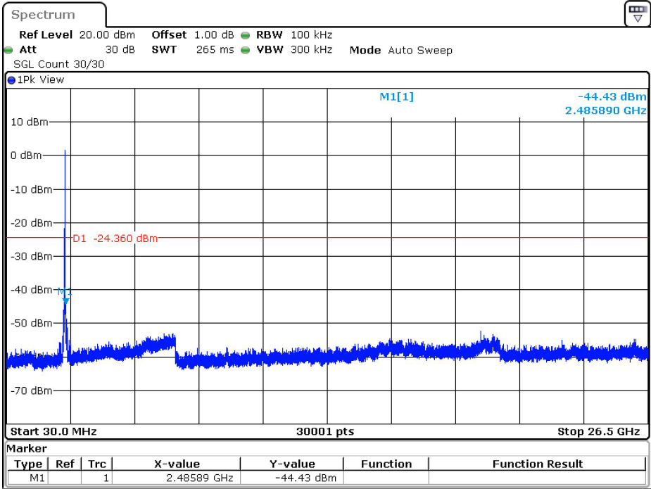
Channel 06 (2437MHz)
