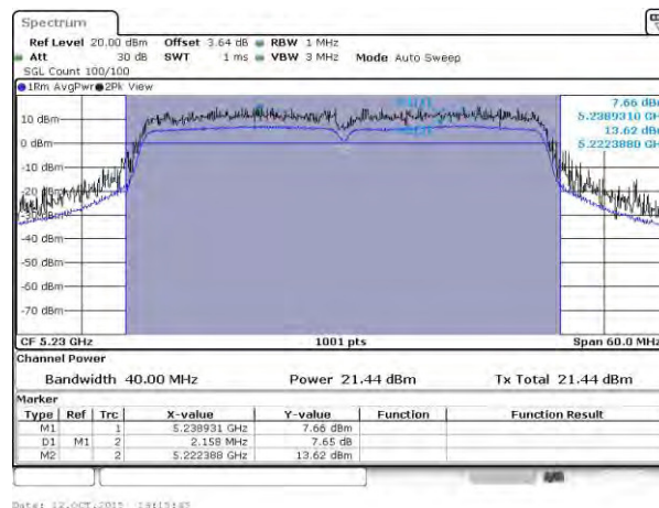
5150-5250MHz - Worst RF Output Power Plots
