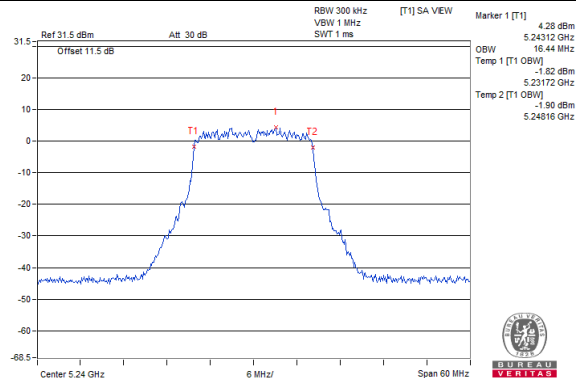
802.11ax (HT20) / Chain 1 / CH 48
