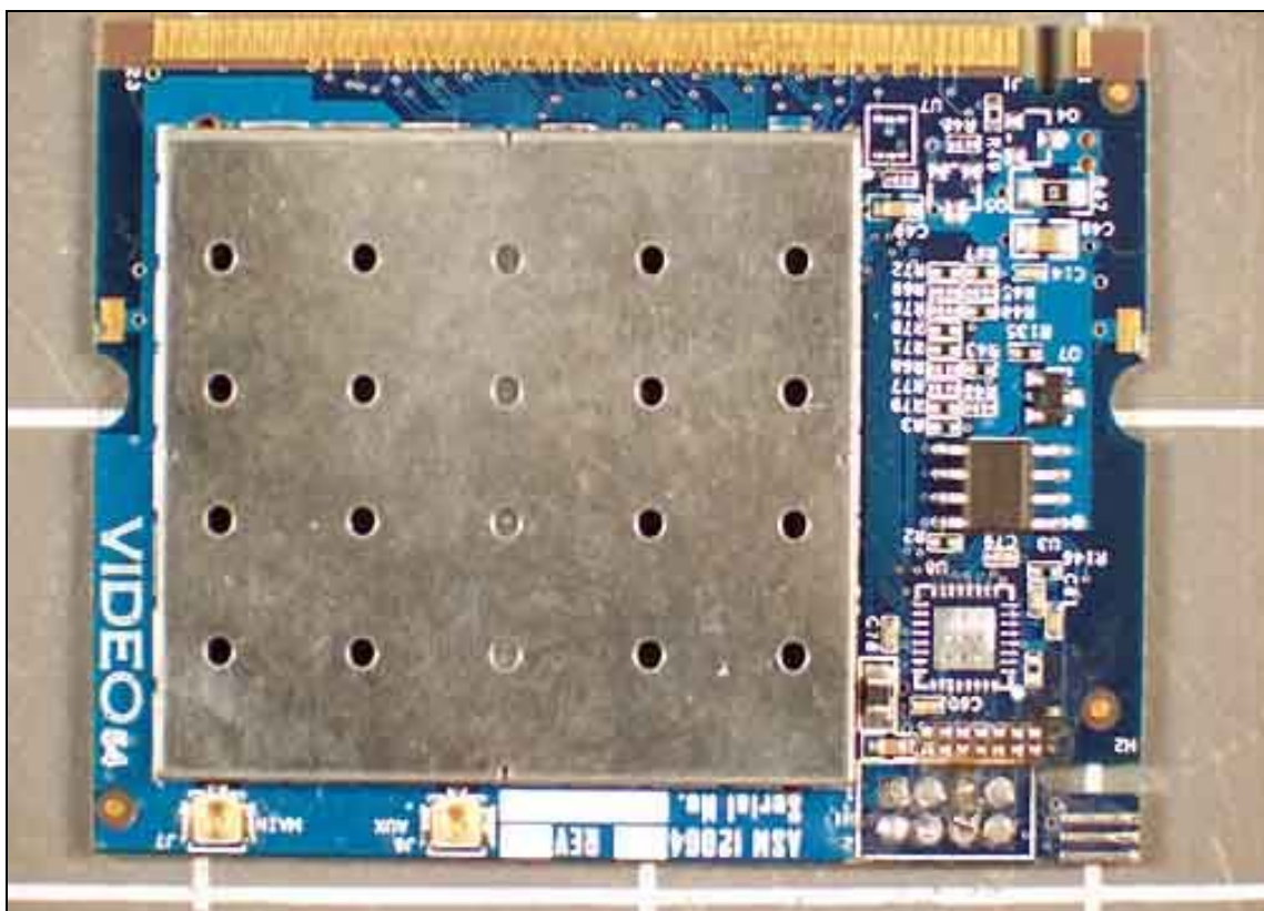
Transmitter Top
