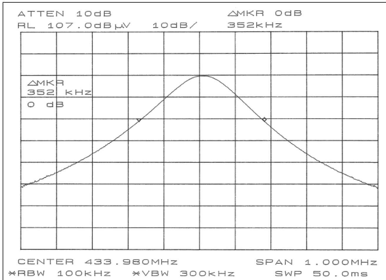
Figure 6.5.3-1: Bandwidth Limitation
