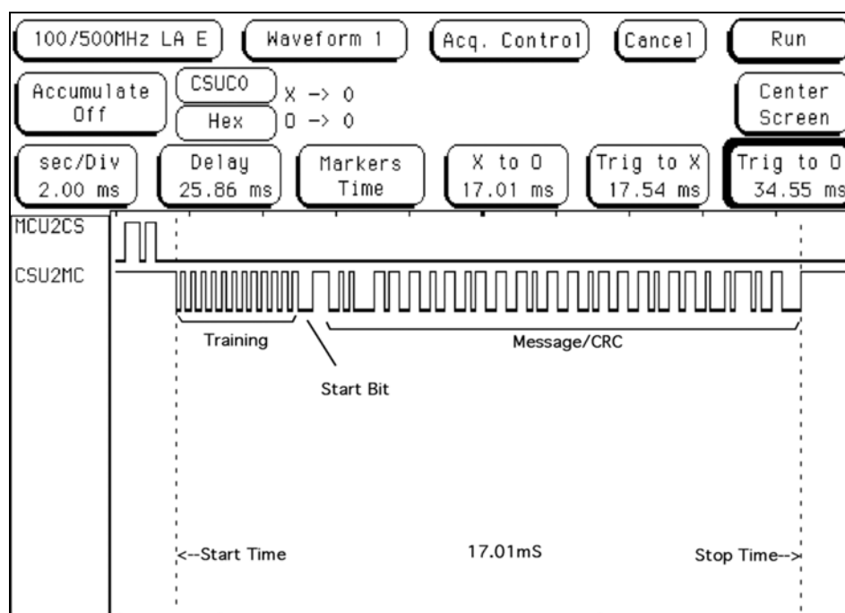
Figure 6.3.3-1: Transmission Duration Timing Diagram
