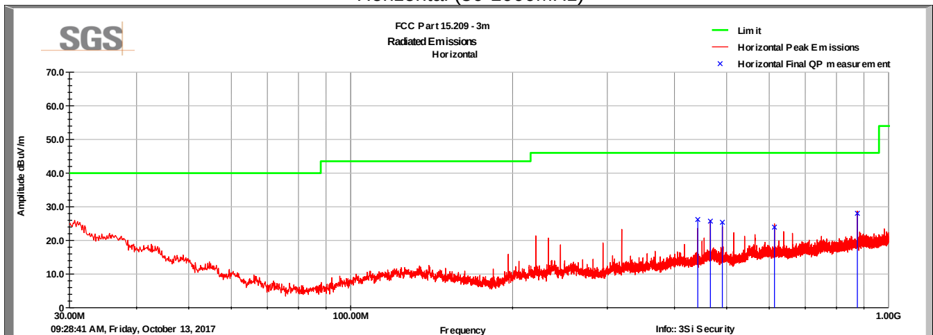
BLE Channel 0 Horizontal (30-1000MHz)
