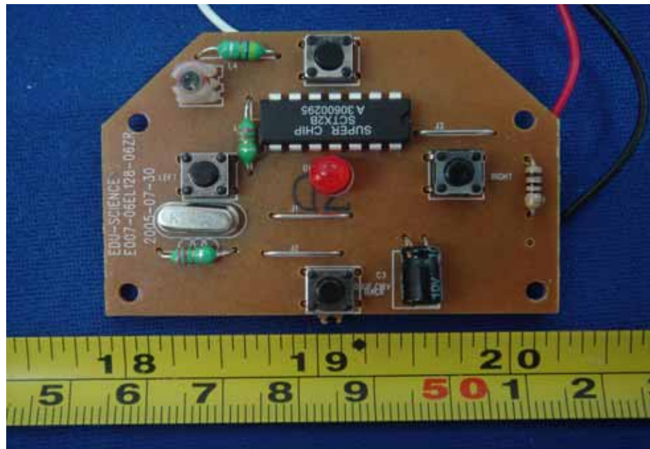
PCB – Component View
