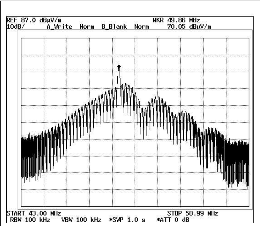
Photo 1 (Rx characteristic)
