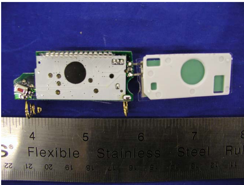
EUT – Solder View 2
