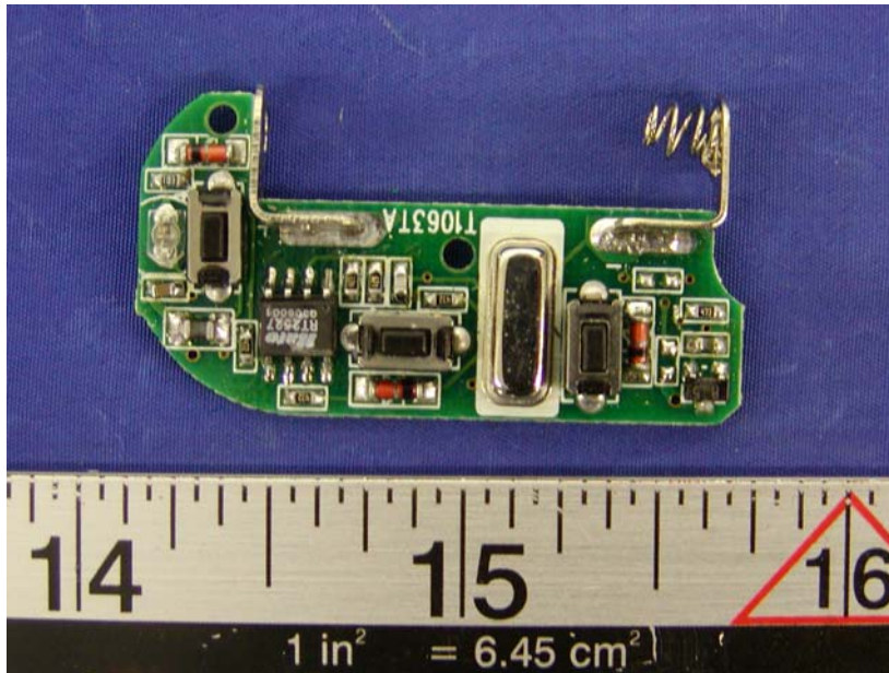
EUT Component View
