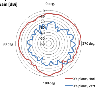
Antenna gain [UNIT: dBi]
