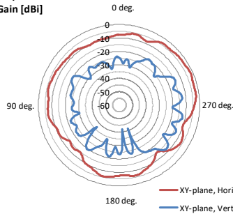
Antenna pattern (Top view)
