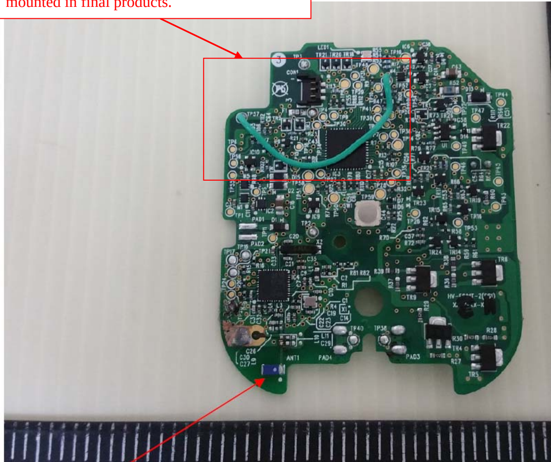
Chip Antenna
