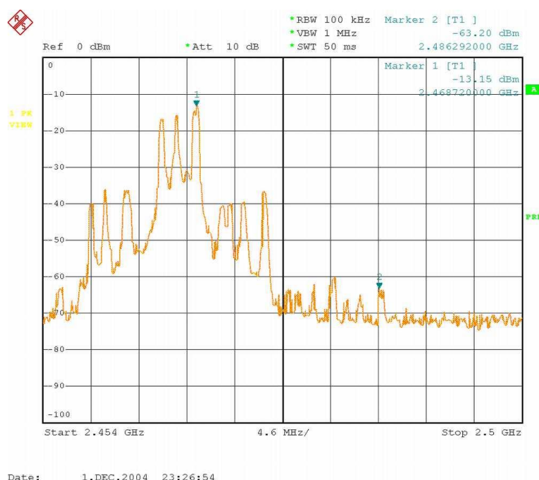
CH4: 2468MHz
