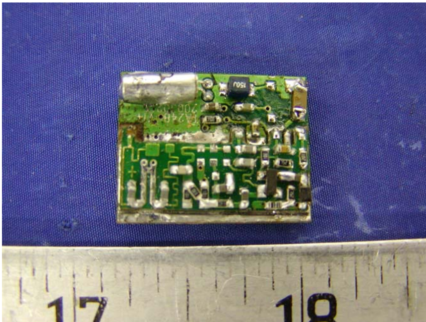
ZT-809 Transmitter – Solder View with Shielded Removed
