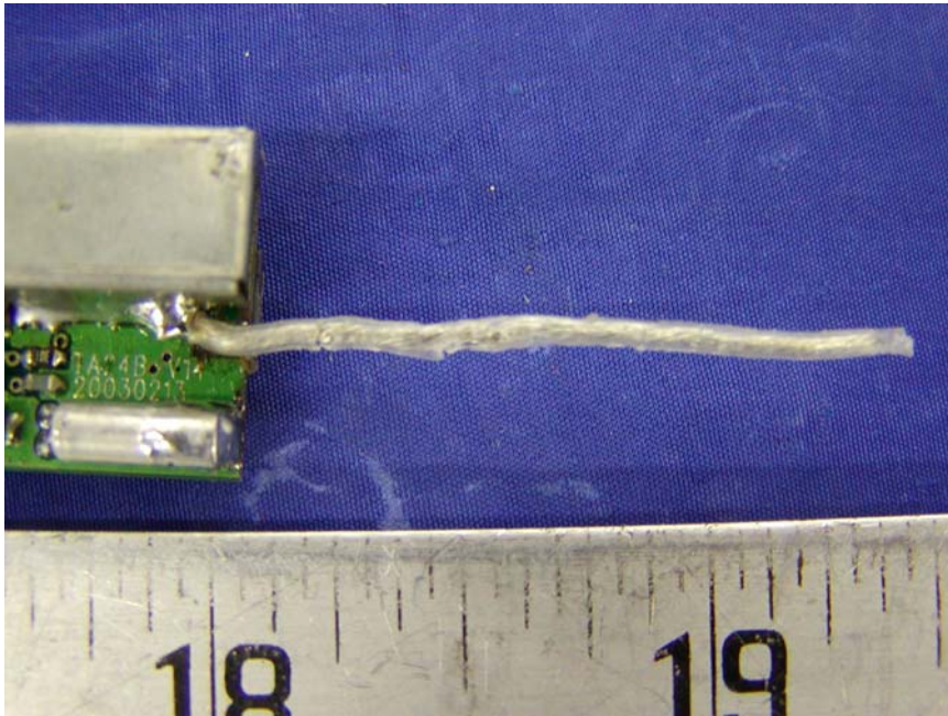
ZT-809 Transmitter – Antenna Connection View
