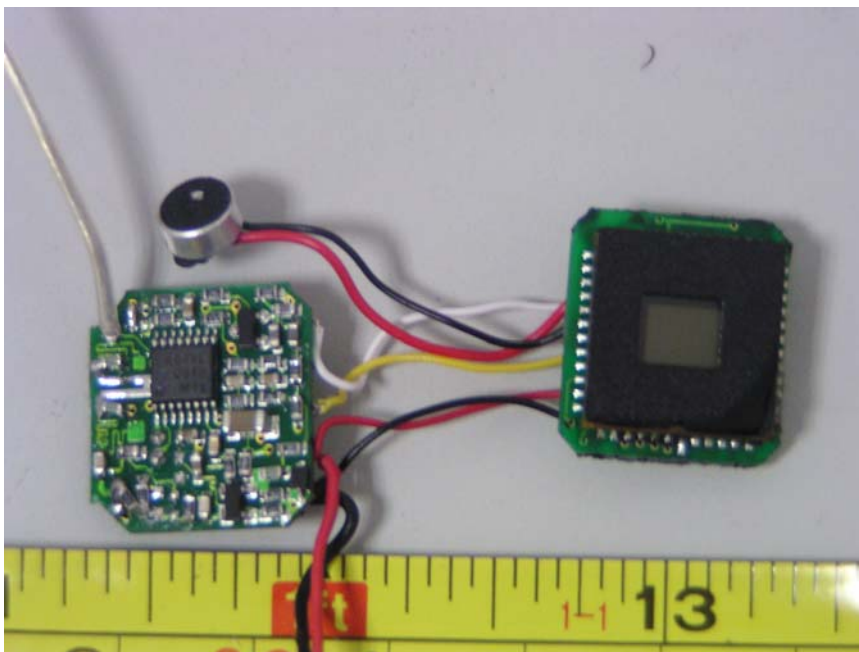
ZT-811 Transmitter Component View
