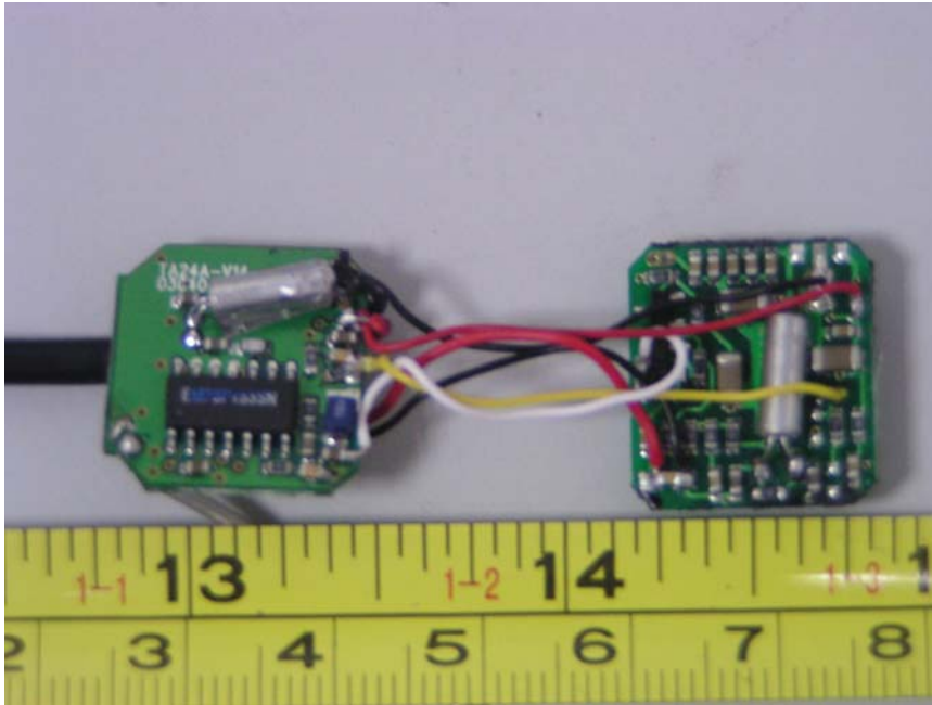
ZT-811 Transmitter Solder View
