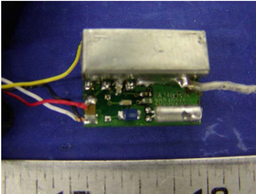
ZT-809 Transmitter – Solder View
