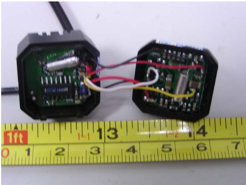
ZT-811 Transmitter Cover Off View
