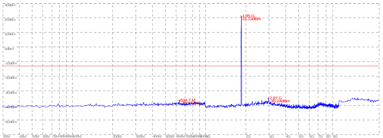
(Plot J: WCDMA 1900MHz Channel = 810, 30MHz to 20GHz)
