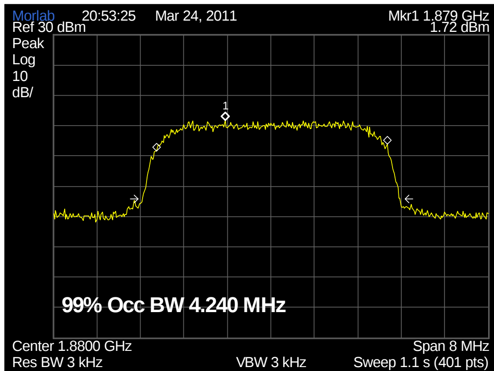
(Plot H: WCDMA 1900MHz Channel = 9400)
