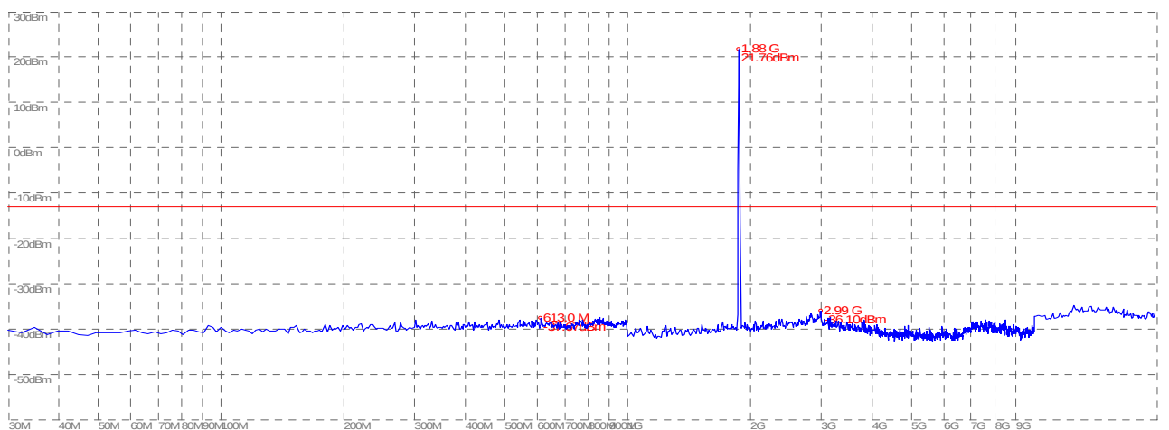
(Plot K: WCDMA 1900MHz Channel = 810, 30MHz to 20GHz)
