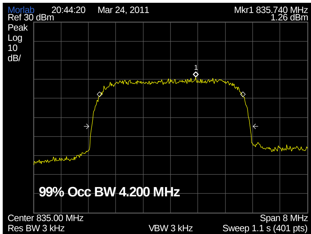
(Plot G: WCDMA 850MHz Channel = 4175)
