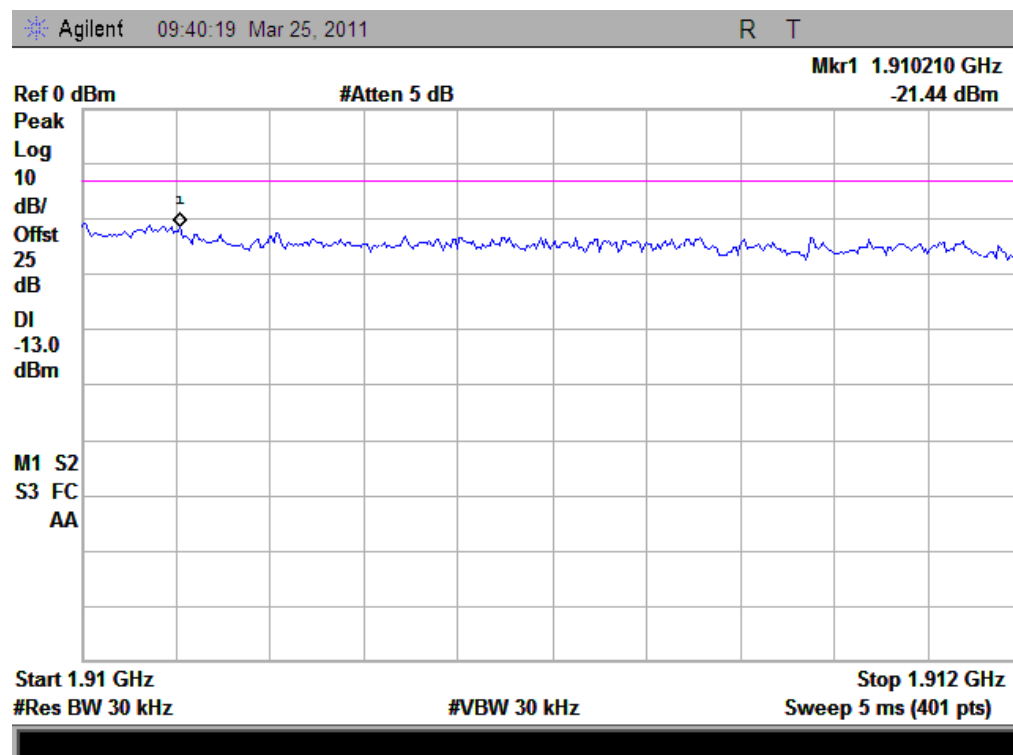
(Plot H: Channel = 810)
