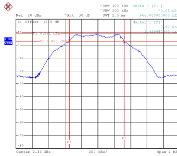
CH19 6 dB Bandwidth
