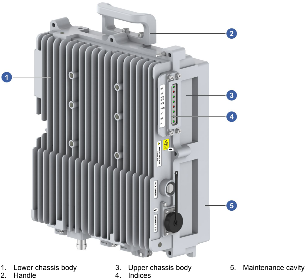
Figure 2-1 External View
