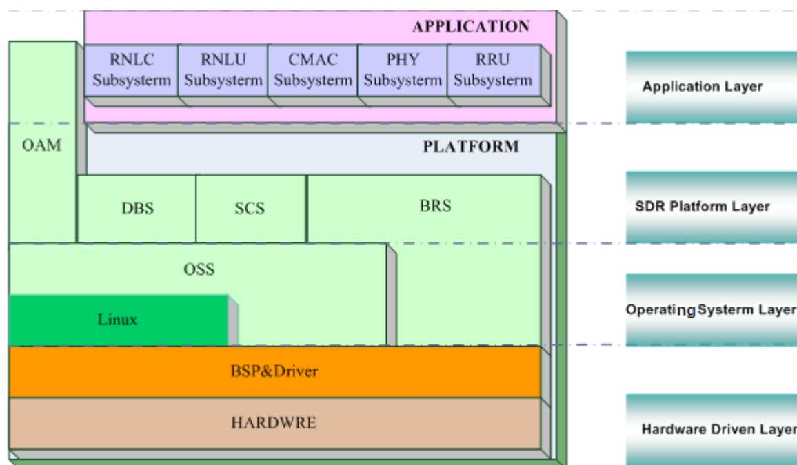
Figure 2-2 Software Architecture
