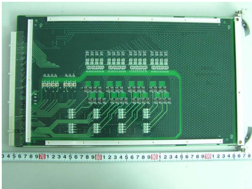
BIM PCB Bottom View
