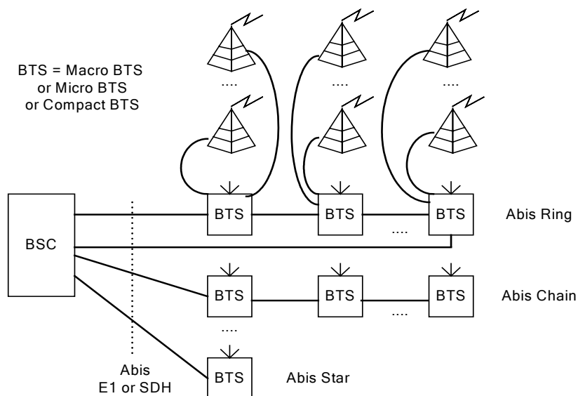
FIG. 12 CDMA2000 BSS NETWORKING
