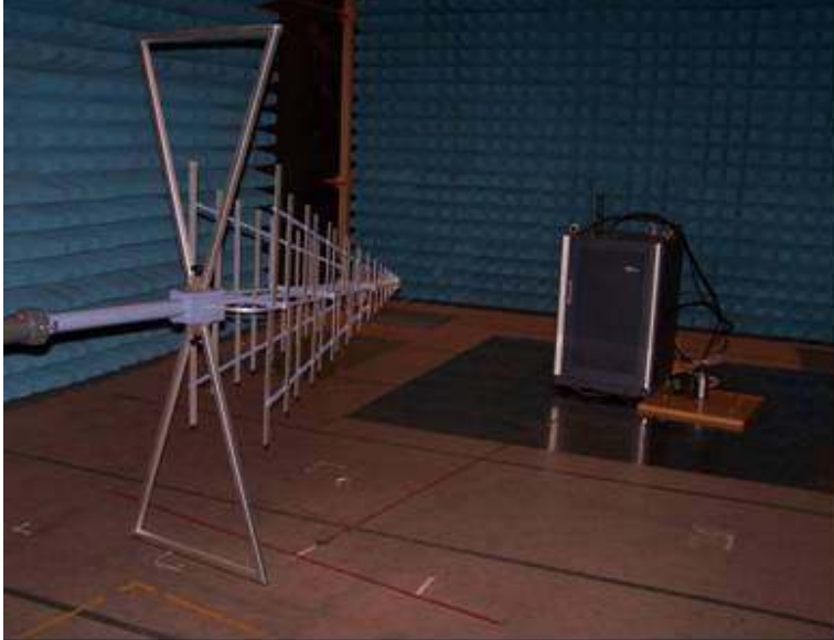
Radiated Emissions-Front View (below 1GHz)
