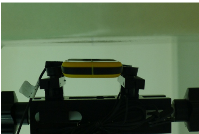
Front of the DUT with Phantom 1.5 cm Gap (With Headset)
