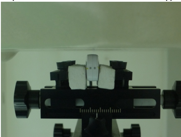
USB Cable Plug-in USB Configuration 4 (Vertical Back with Phantom 0.5 cm Gap)
