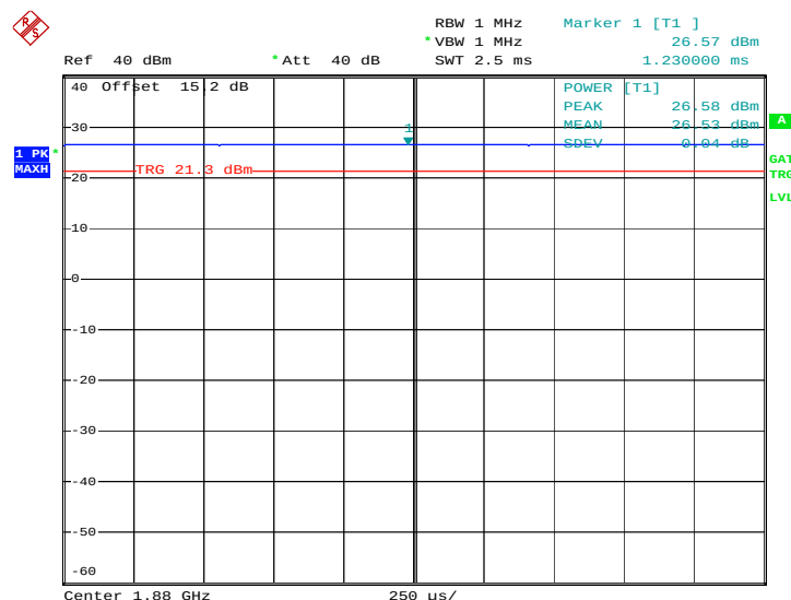
Peak-to-Average Ratio on Channel 661 (1880.0 MHz)
