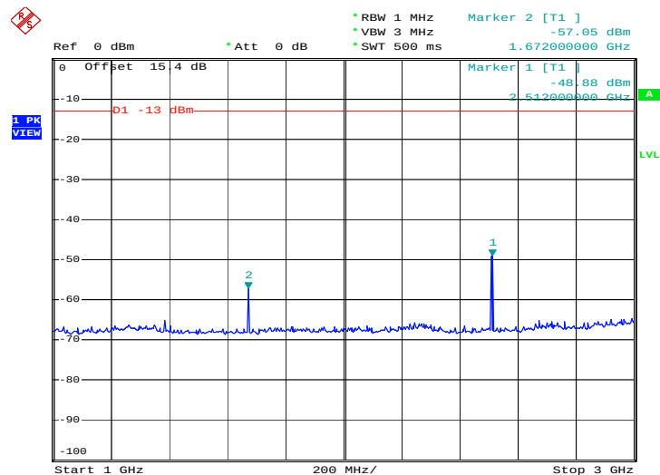
Conducted Spurious Emission Plot between 1GHz ~ 3GHz
