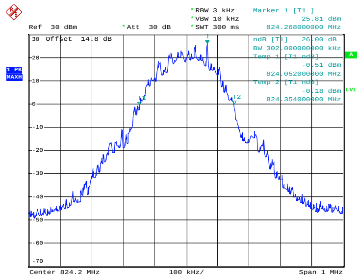
26dB Bandwidth Plot on Channel 128 (824.2 MHz)
