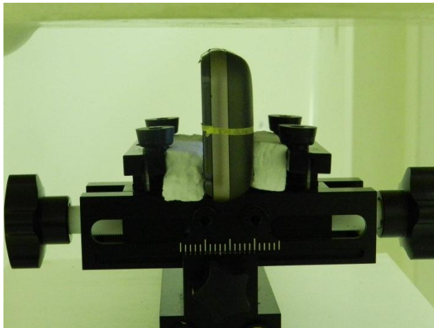
Bottom of the DUT with Phantom 1 cm Gap
