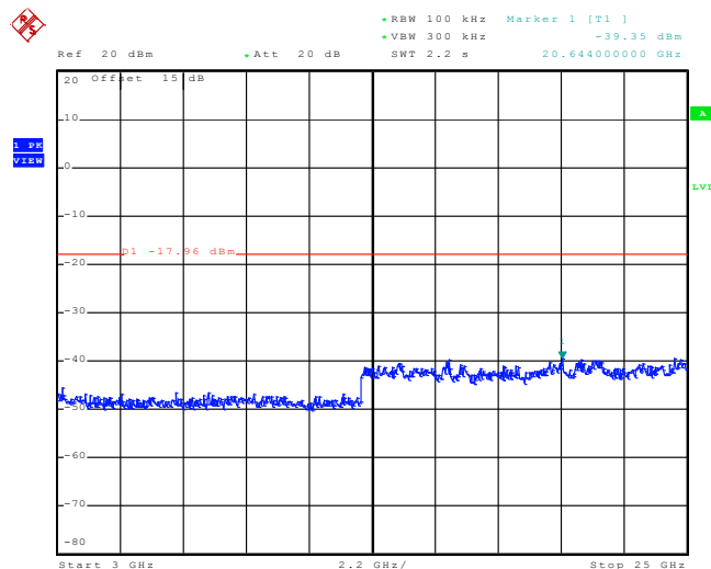
Conducted Spurious Emission Plot between 3 GHz ~ 25 GHz
