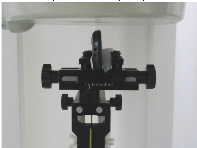
Right Side with Phantom 1 cm Gap (DUT without Earphone)
