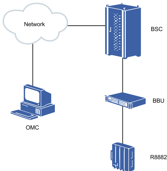
Figure 3-1 Remote Maintenance Mode (Taking CDMA and GSM for Example)
