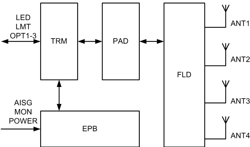
Figure 2-1 ZXSDR R8882 Hardware Subsystem
