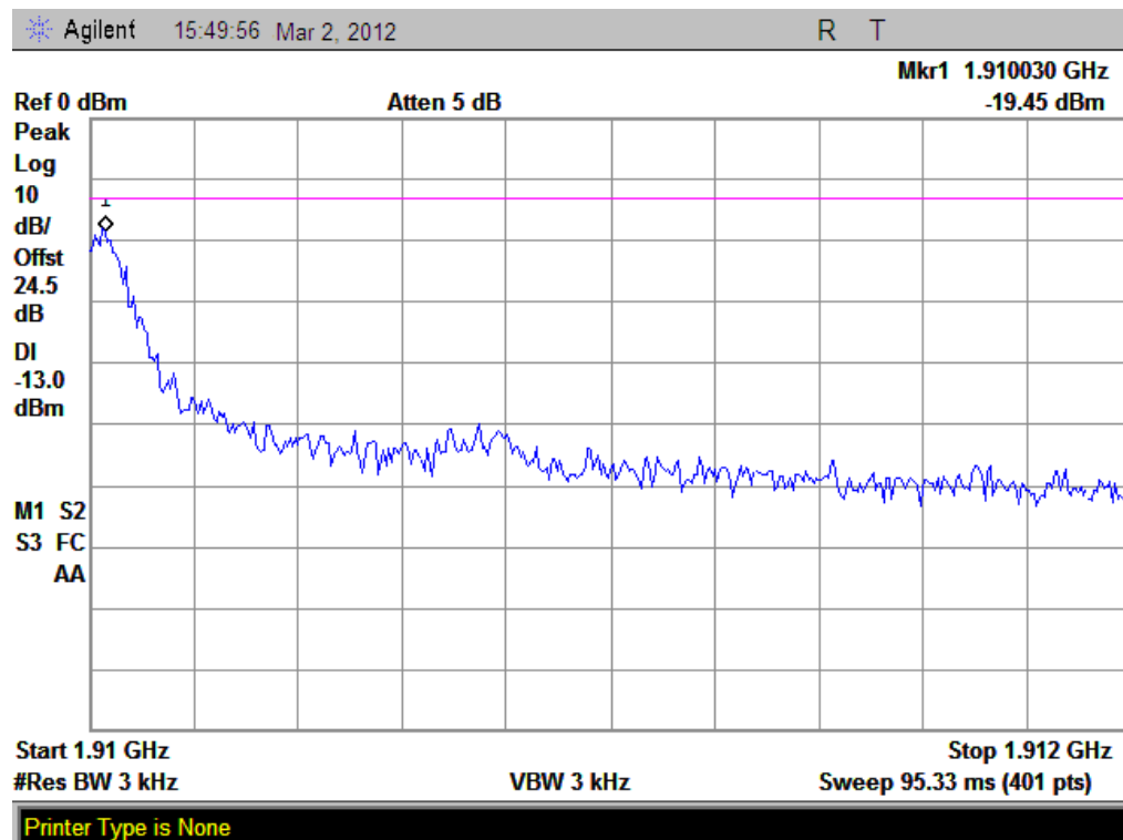
(Plot T: GPRS 1900 Channel = 810)
