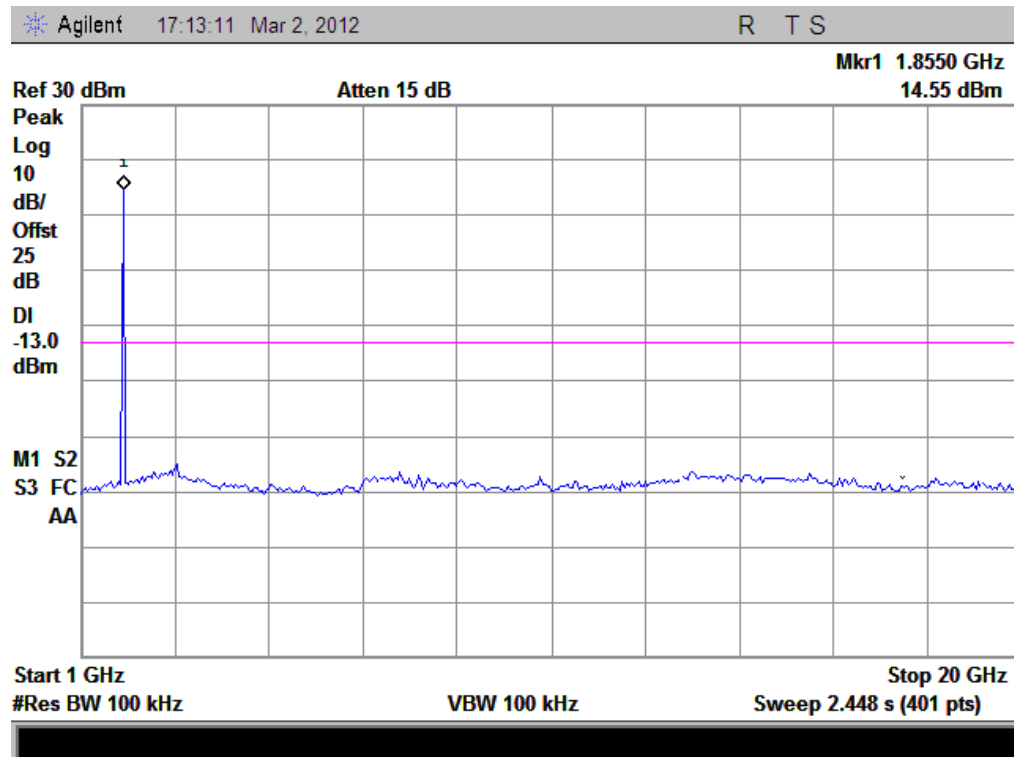
(Plot D1.1: WCDMA1900MHz Channel = 9262, 1GHz to 20GHz)
