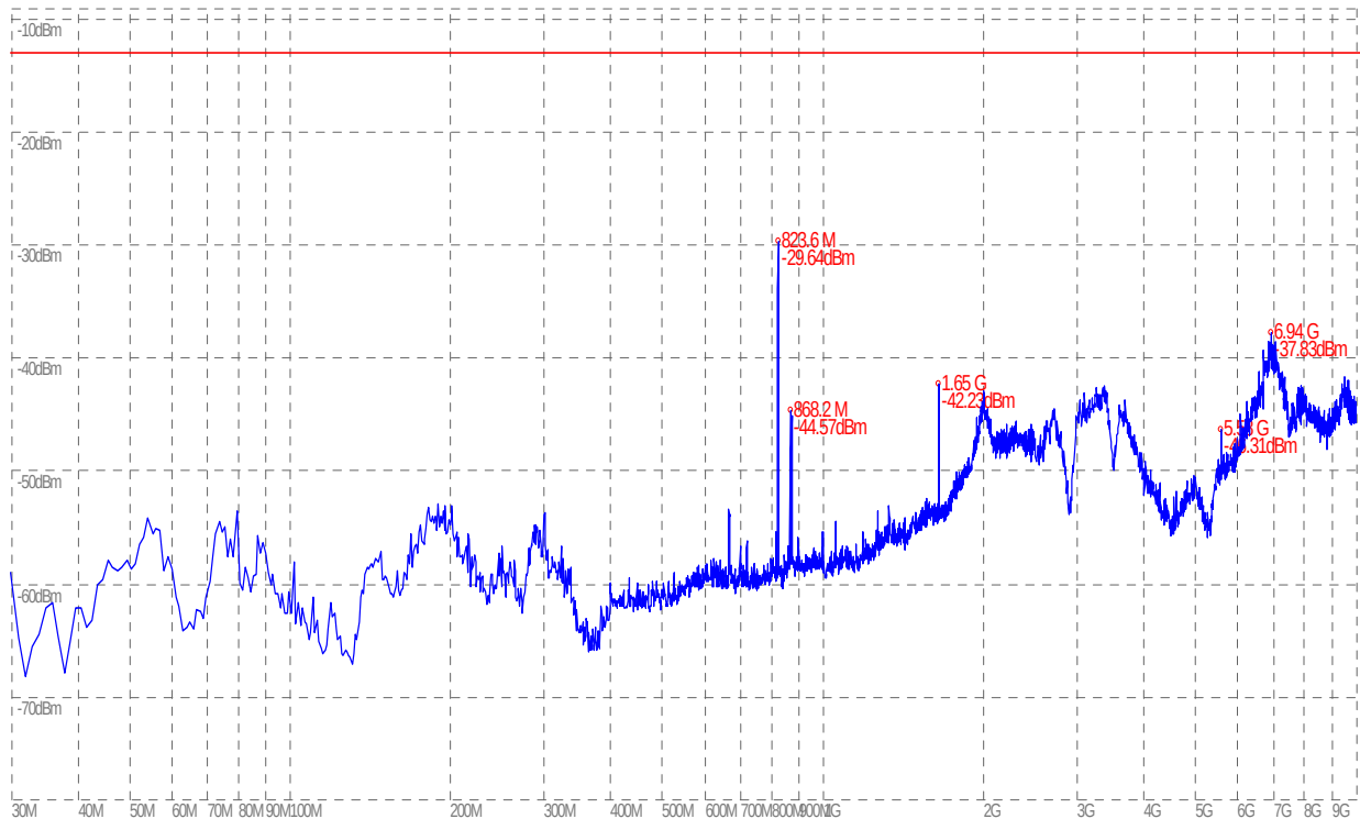
(Plot A.2: EGPRS 850MHz Channel = 128, Test Antenna Vertical)
