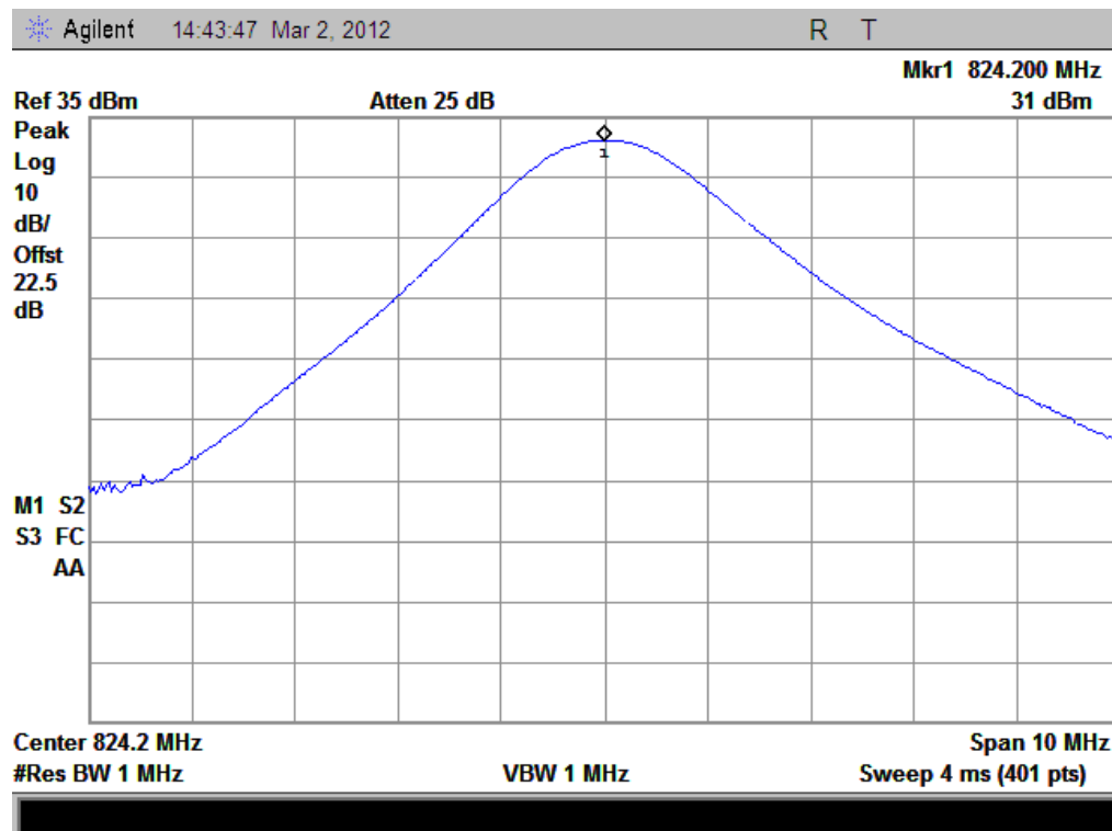
(Plot A1: GPRS 850MHz Channel = 128)
