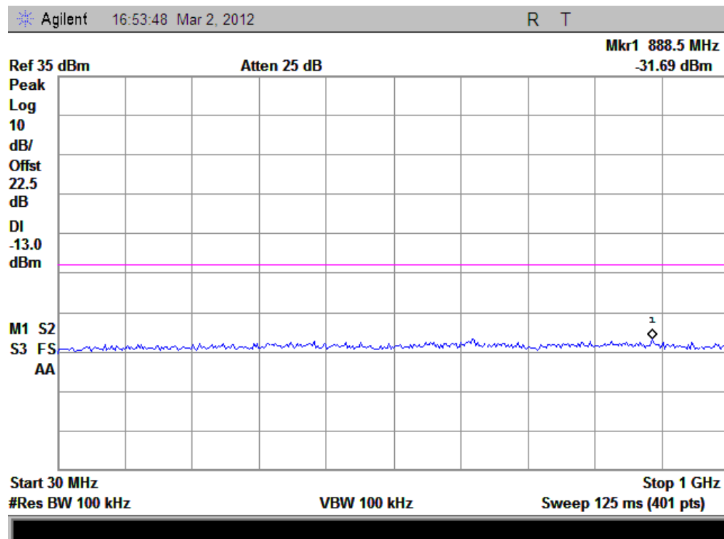
(Plot D3: WCDMA1900MHz Channel = 9538, 30MHz to 1GHz)
