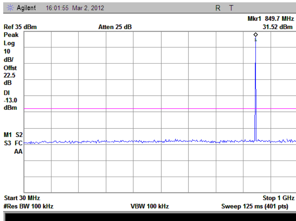
(Plot A3: EDGE 850MHz Channel = 251, 30MHz to 1GHz)
