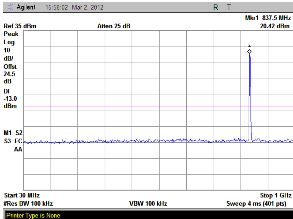
(Plot I 2: GPRS 850MHz Channel = 190, 30MHz to 1GHz)
