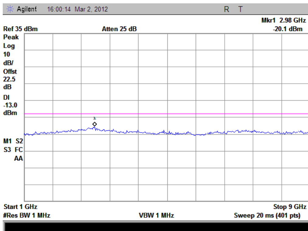
(Plot A3.1: EDGE 850MHz Channel = 251, 1GHz to 9GHz)
