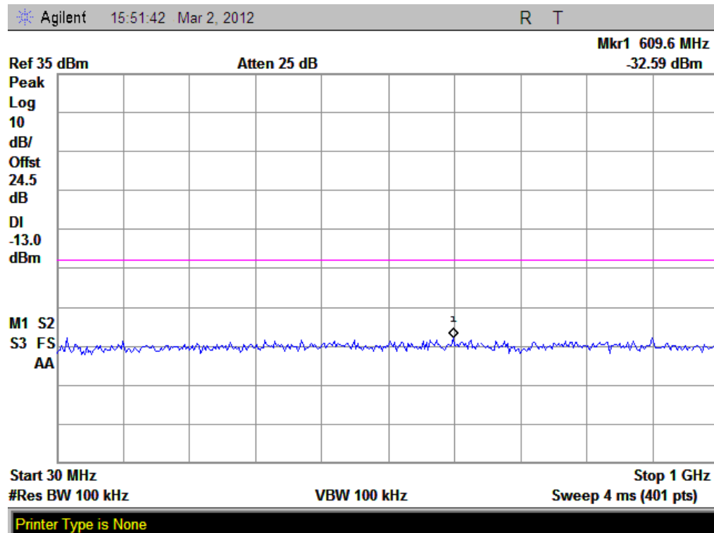
(Plot J 1: GPRS 1900MHz Channel = 512, 30MHz to 1GHz)
