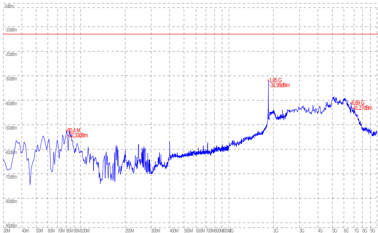
(Plot D.2: WCDMA 1900MHz Channel = 9262, Test Antenna Vertical)
