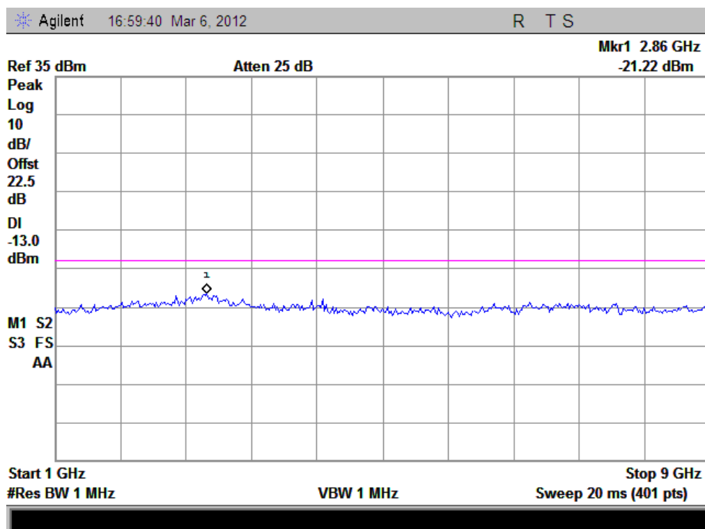
(Plot E 3.1: HSDPA850MHz Channel = 4233, 1GHz to 9GHz)
