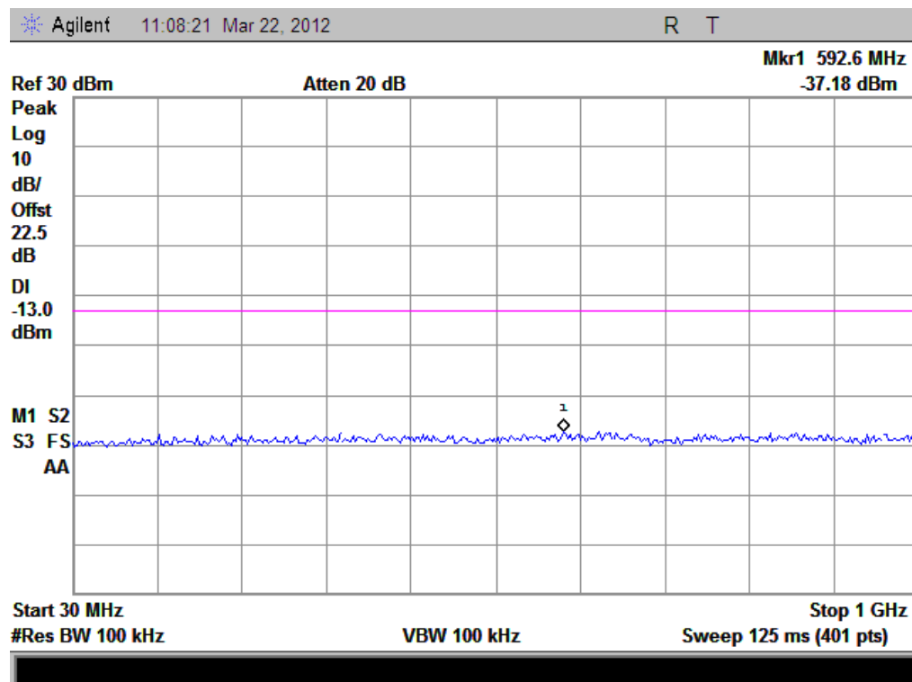
(Plot H 2: HSUPA1900MHz Channel = 9400, 30MHz to 1GHz)
