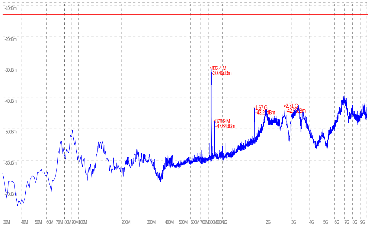
(Plot E.5: HSDPA 850MHz Channel = 4233, Test Antenna Horizontal)
