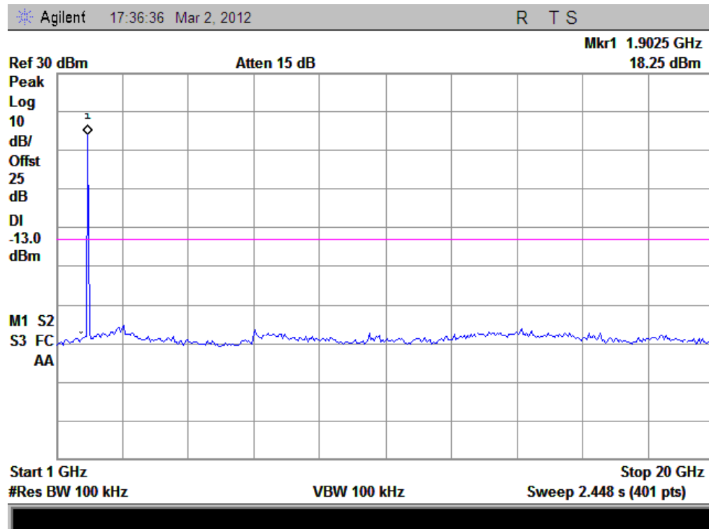
(Plot F3.1: HSDPA1900MHz Channel = 9538 1GHz to 20GHz)
