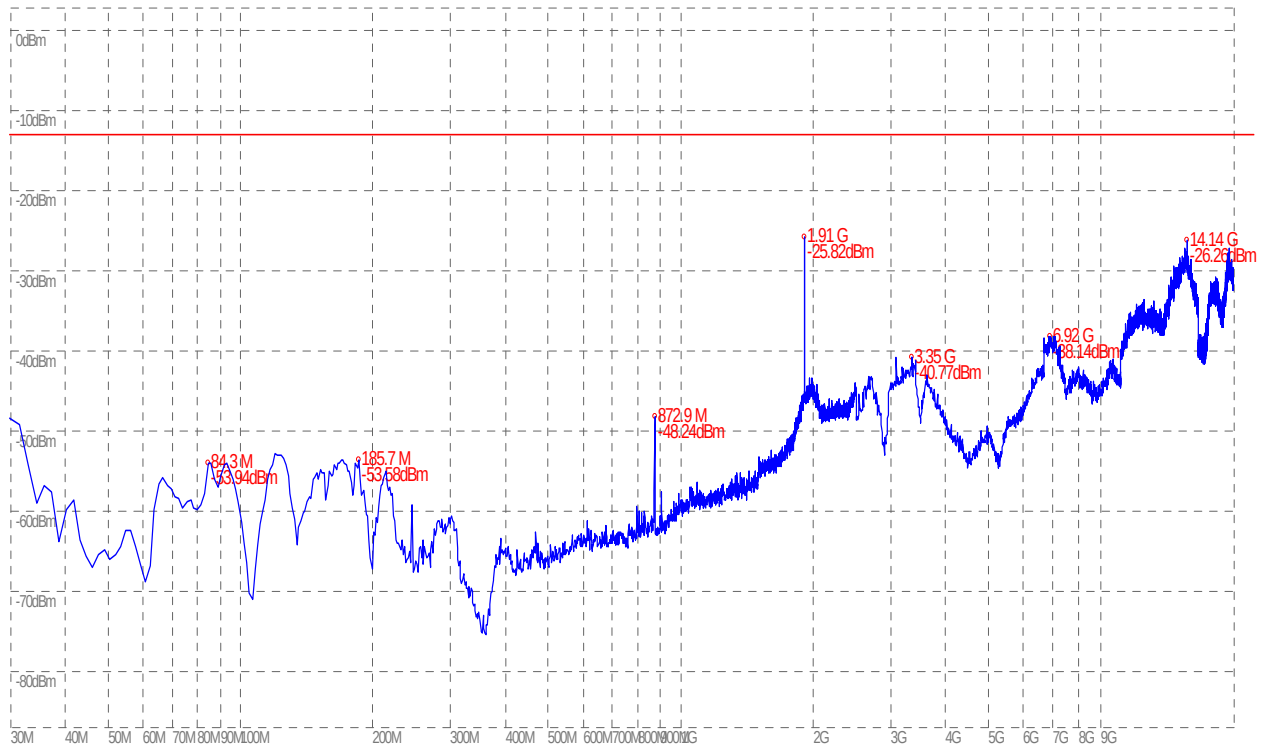
(Plot J.6: GPRS 1900MHz Channel = 810, Test Antenna Vertical)
