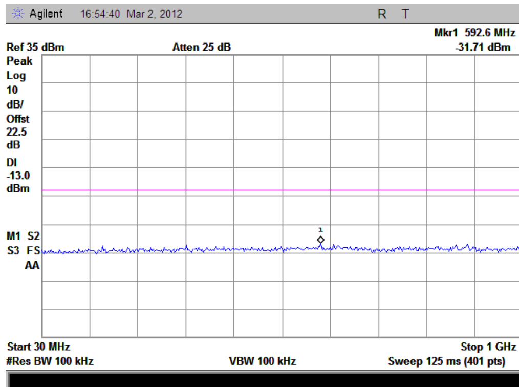
(Plot D2: WCDMA1900MHz Channel = 9400, 30MHz to 1GHz)
