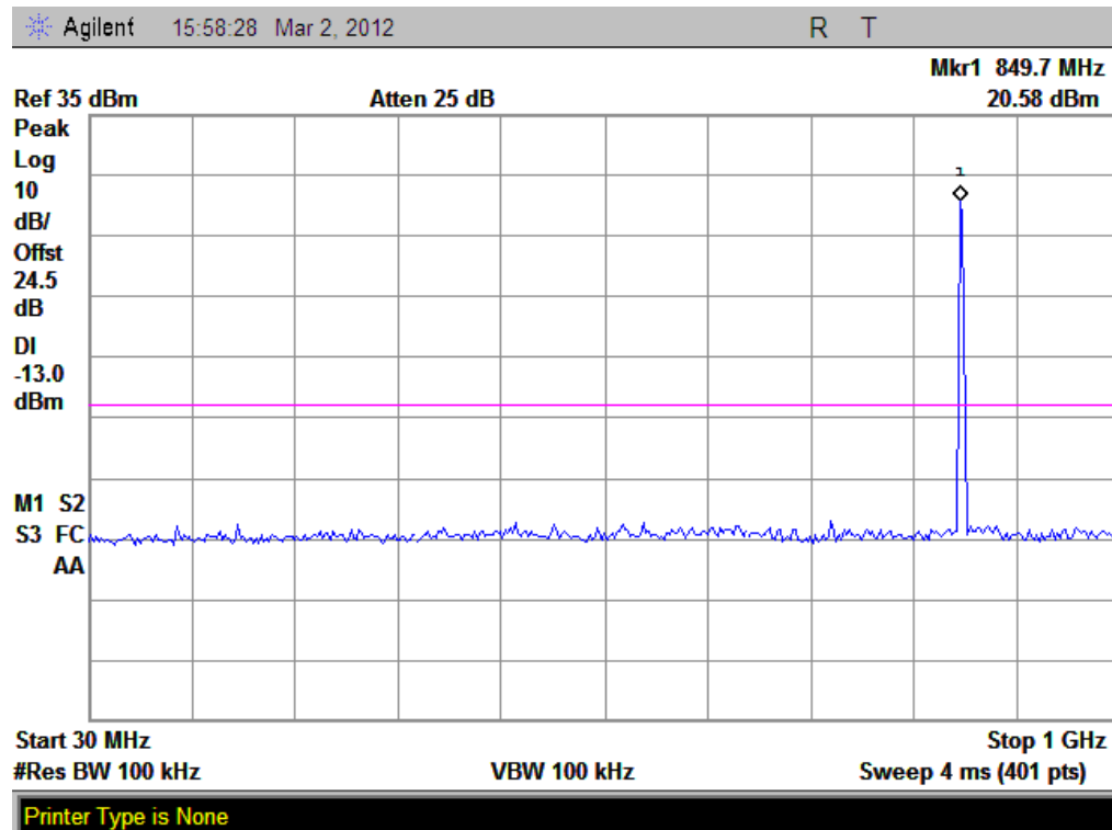
(Plot I 3: GPRS 850MHz Channel = 251, 30MHz to 1GHz)
