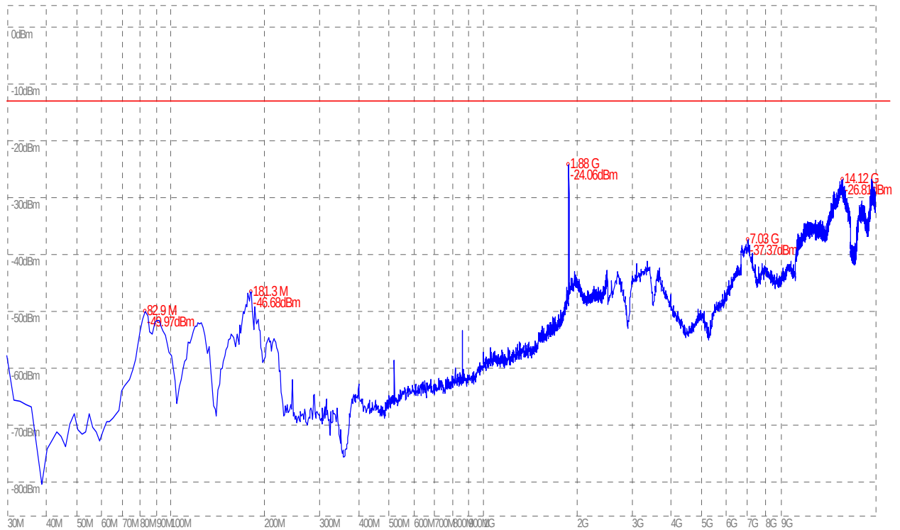
(Plot J.3: GPRS1900MHz Channel = 661, Test Antenna Horizontal)
