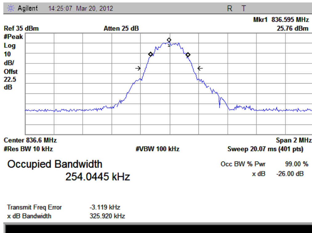
(Plot N: GPRS 850MHz Channel = 190)
