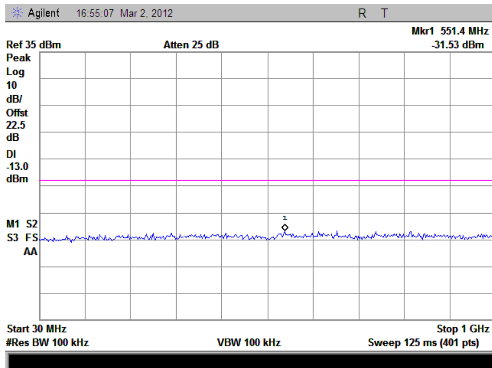
(Plot D1: WCDMA1900MHz Channel = 9262, 30MHz to 1GHz)
