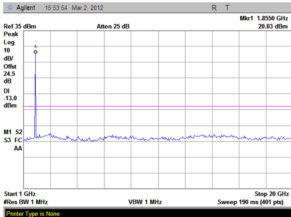
(Plot J 1.1: GPRS 1900MHz Channel = 512, 1GHz to 20GHz)
