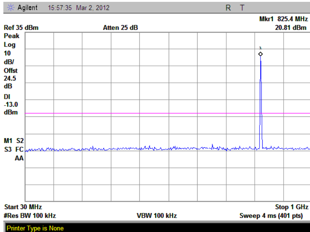
(Plot I 1: GPRS 850MHz Channel = 128, 30MHz to 1GHz)
