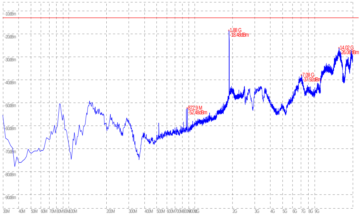
(Plot B.3: EGPRS 1900MHz Channel = 661, Test Antenna Horizontal)
