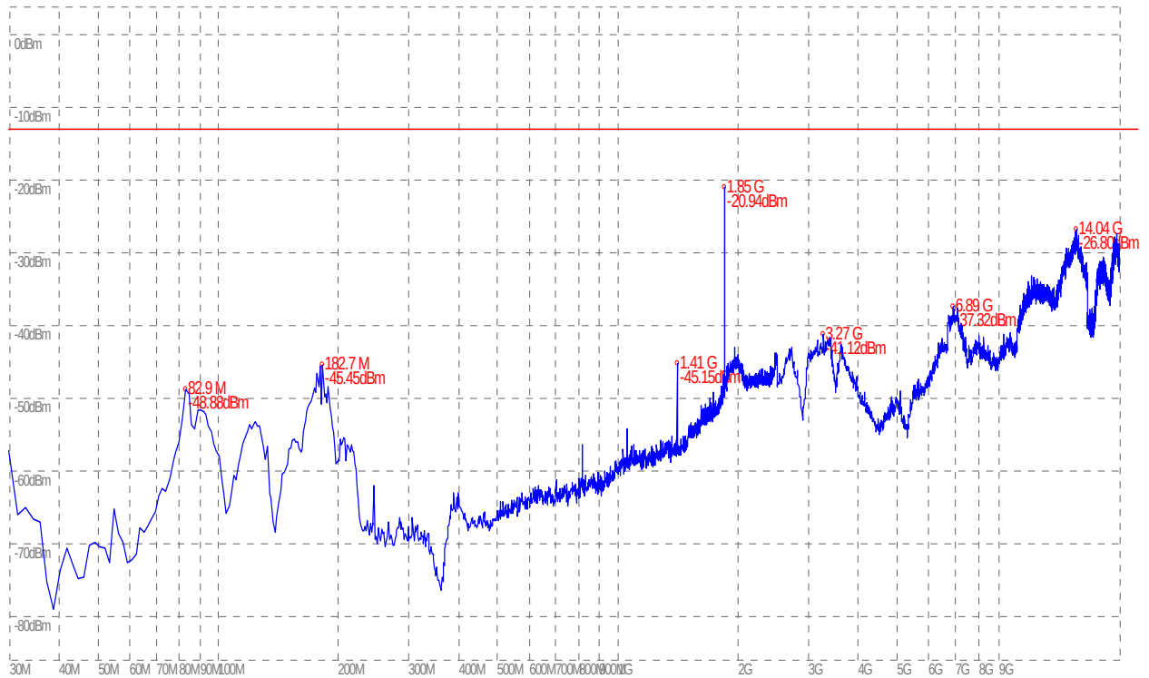
(Plot J.1: GPRS1900MHz Channel = 512, Test Antenna Horizontal)
