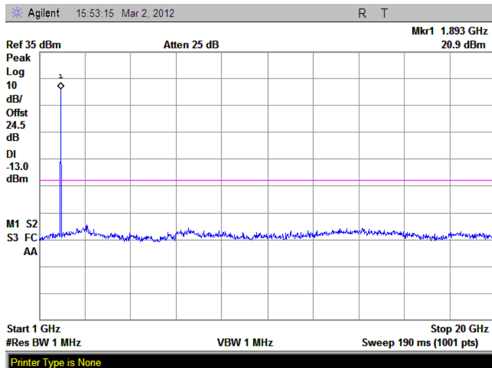
(Plot J 2.1: GPRS 1900MHz Channel = 661, 1GHz to 20GHz)
