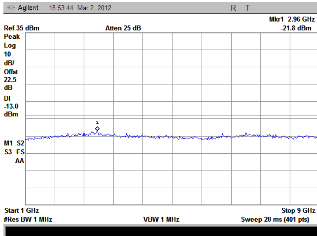
(Plot A2.1: EDGE 850MHz Channel = 190, 1GHz to 9GHz)
