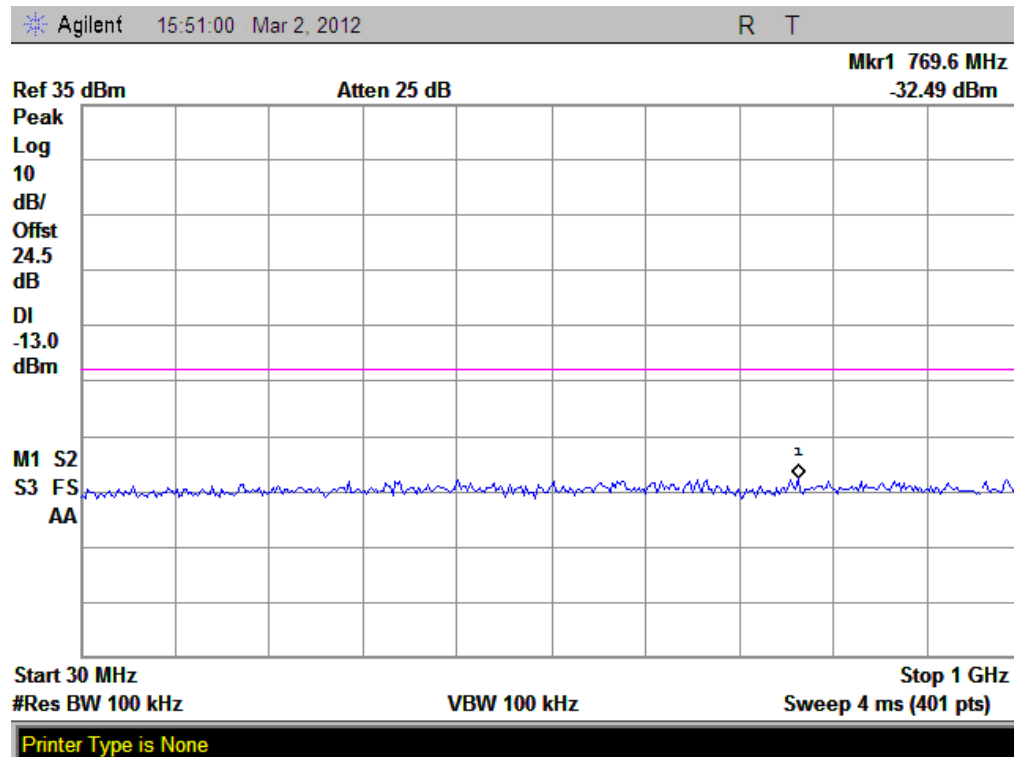
(Plot J 3: GPRS 1900MHz Channel = 810, 30MHz to 1GHz)
