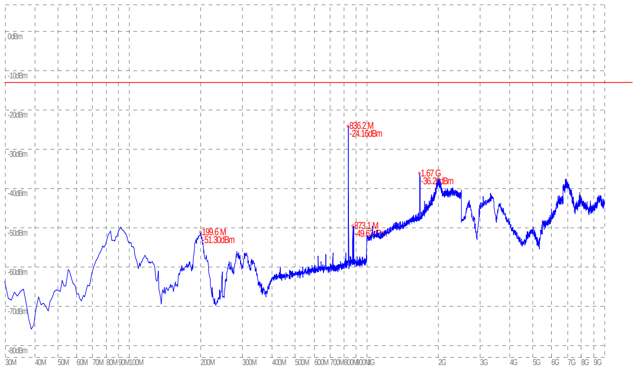
(Plot I.3: GPRS 850MHz Channel = 190, Test Antenna Horizontal)
