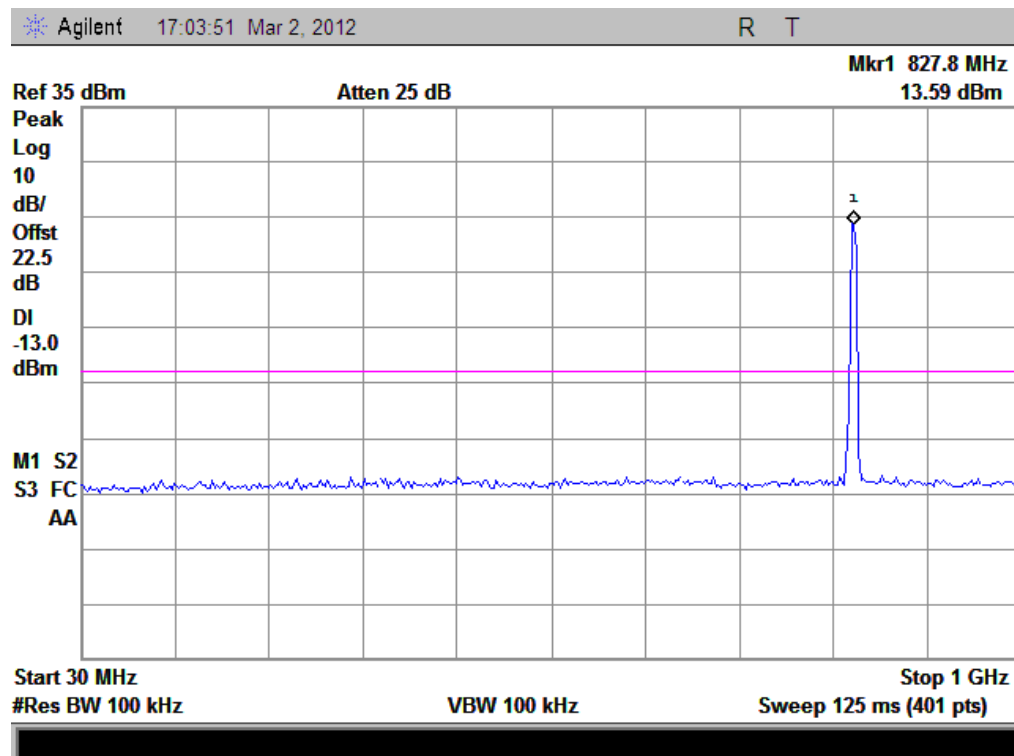
(Plot C1: WCDMA850MHz Channel = 4132, 30MHz to 1GHz)
