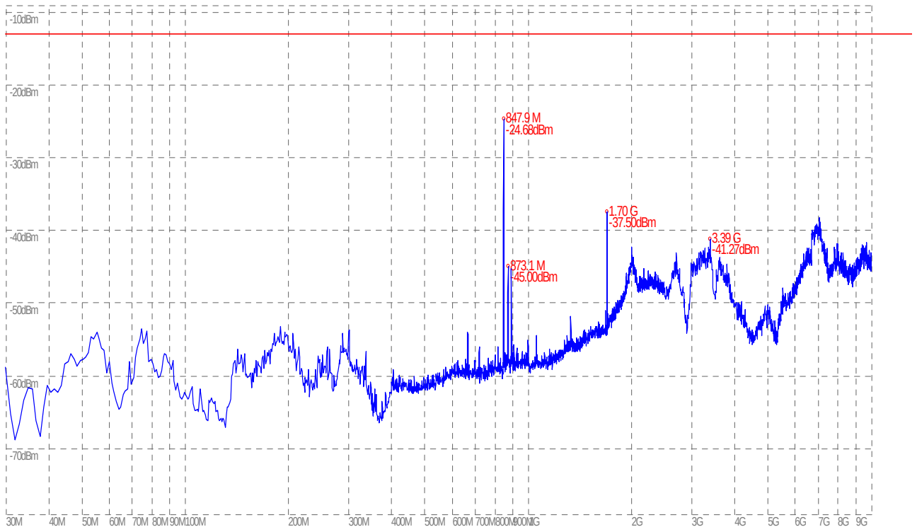
(Plot A.6: EGPRS 850MHz Channel = 251, Test Antenna Vertical)
