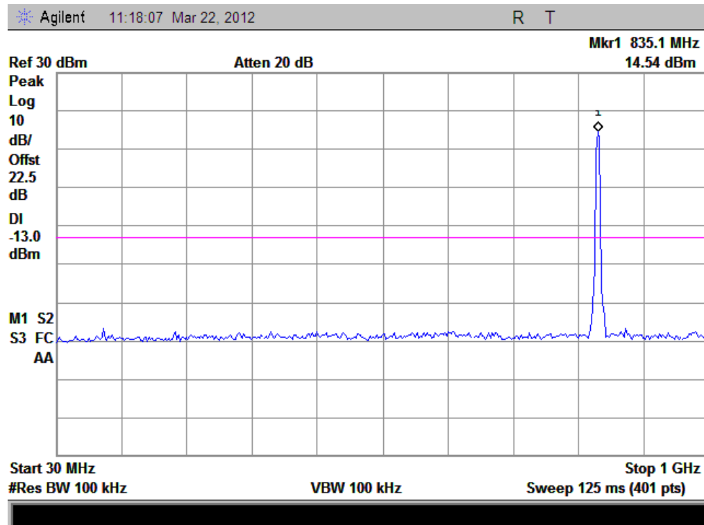
(Plot G 2: HSUPA 850MHz Channel = 4175, 30MHz to 1GHz)
