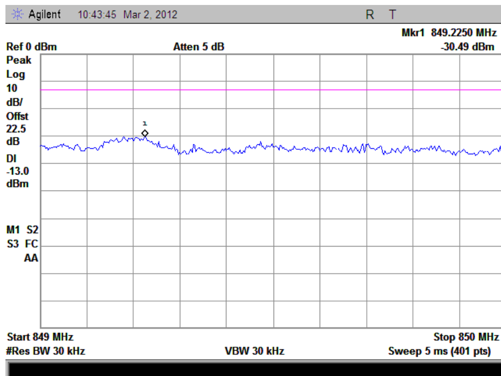
(Plot N: HSUPA850 Channel = 4233)
