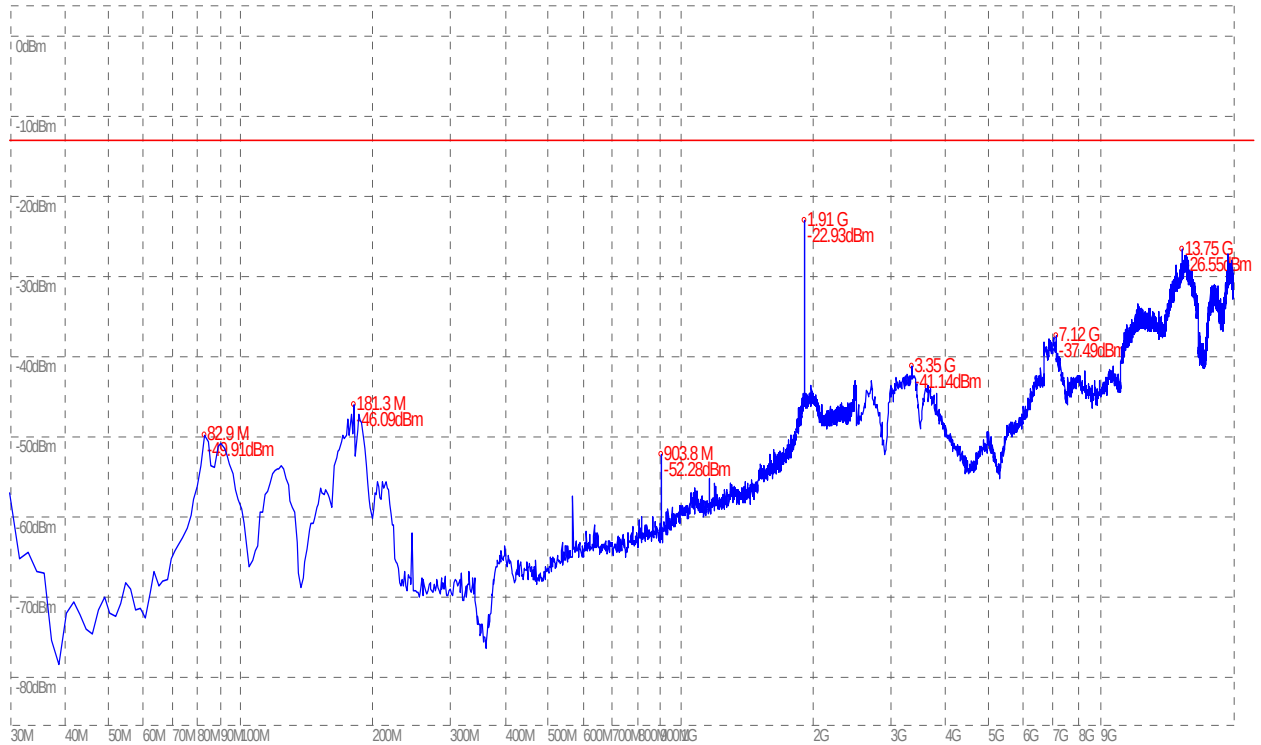
(Plot J.5: GPRS 1900MHz Channel = 810, Test Antenna Horizontal)
