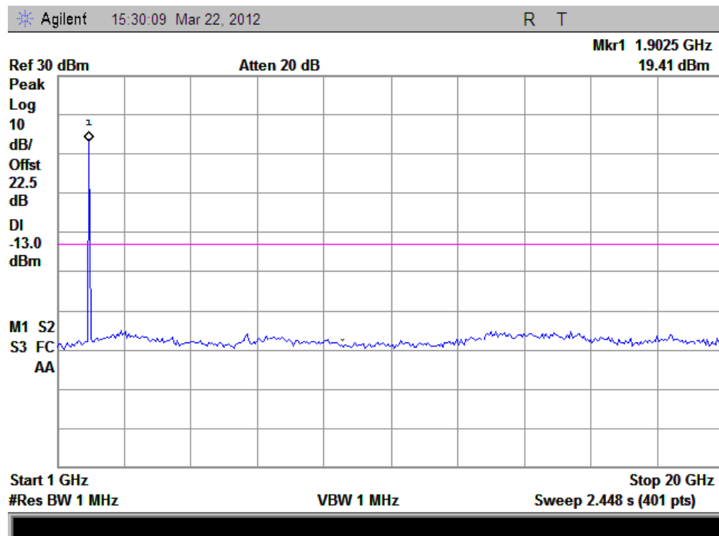
(Plot H3.1: HSUPA1900MHz Channel = 9538 1GHz to 20GHz)
