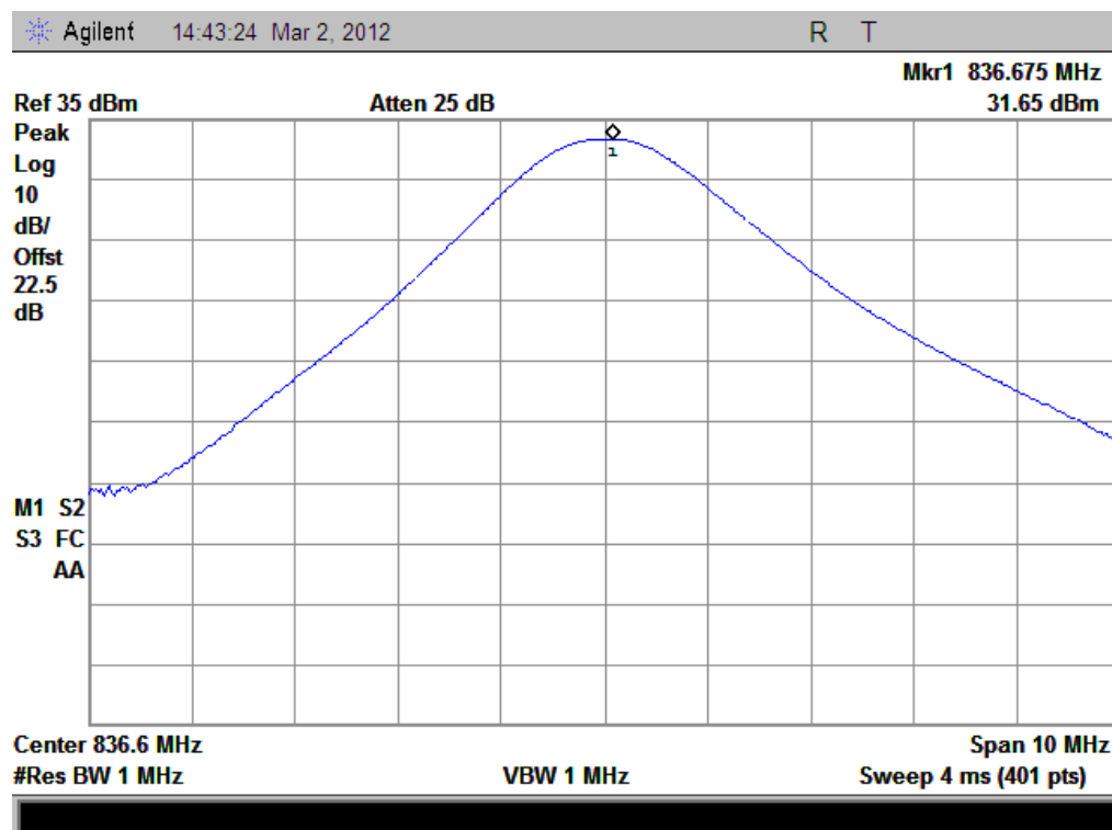
(Plot A2: GPRS 850MHz Channel = 190)
