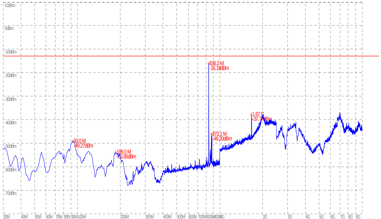
(Plot I.4: GPRS 850MHz Channel = 190, Test Antenna Vertical)
