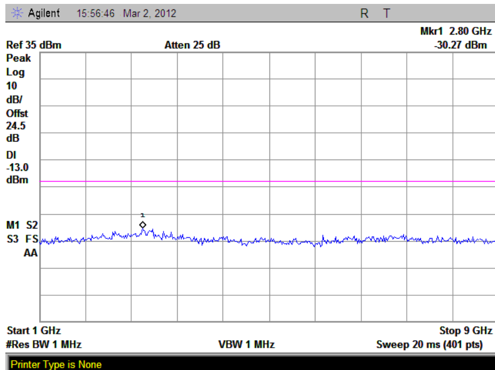
(Plot I3.1: GPRS 850MHz Channel = 251, 1GHz to 9GHz)
