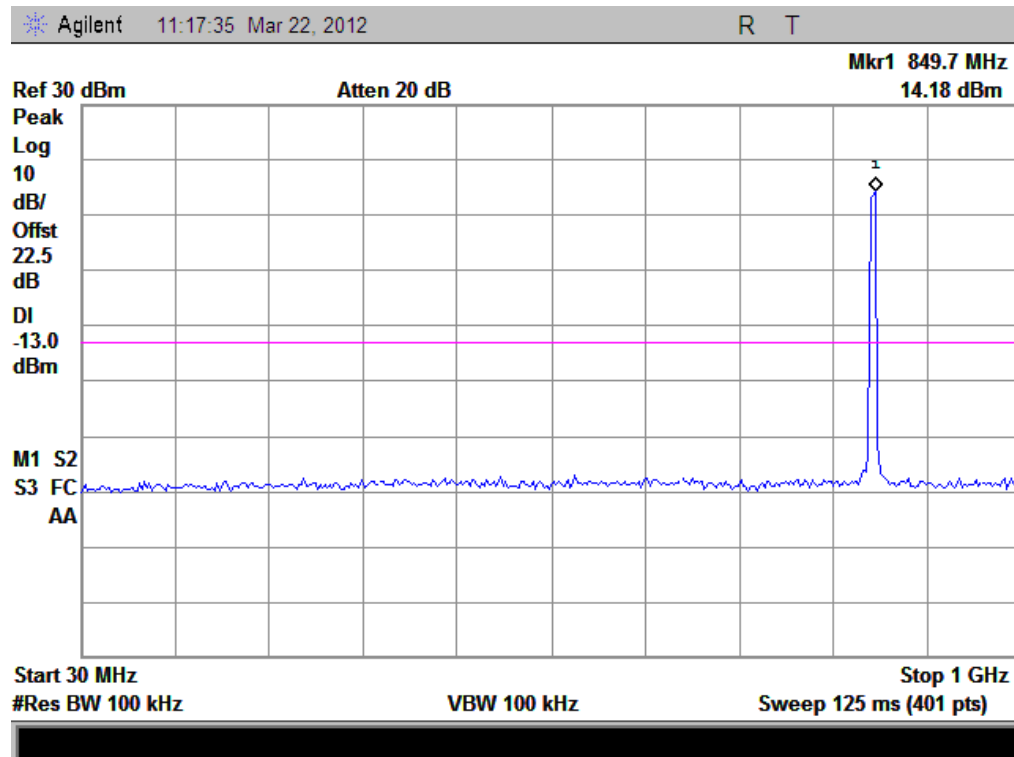
(Plot G 3: HSUPA850MHz Channel = 4233, 30MHz to 1GHz)
