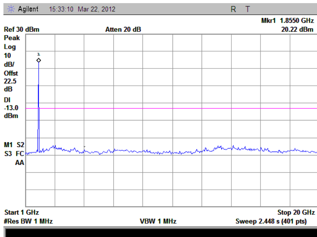
(Plot H1.1: HSUPA1900MHz Channel = 9262, 1GHz to 20GHz)
