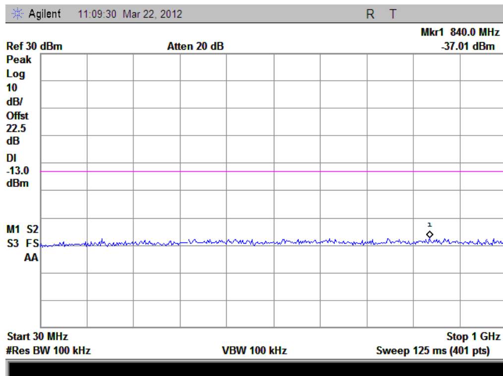
(Plot H 1: HSUPA1900MHz Channel = 9262, 30MHz to 1GHz)
