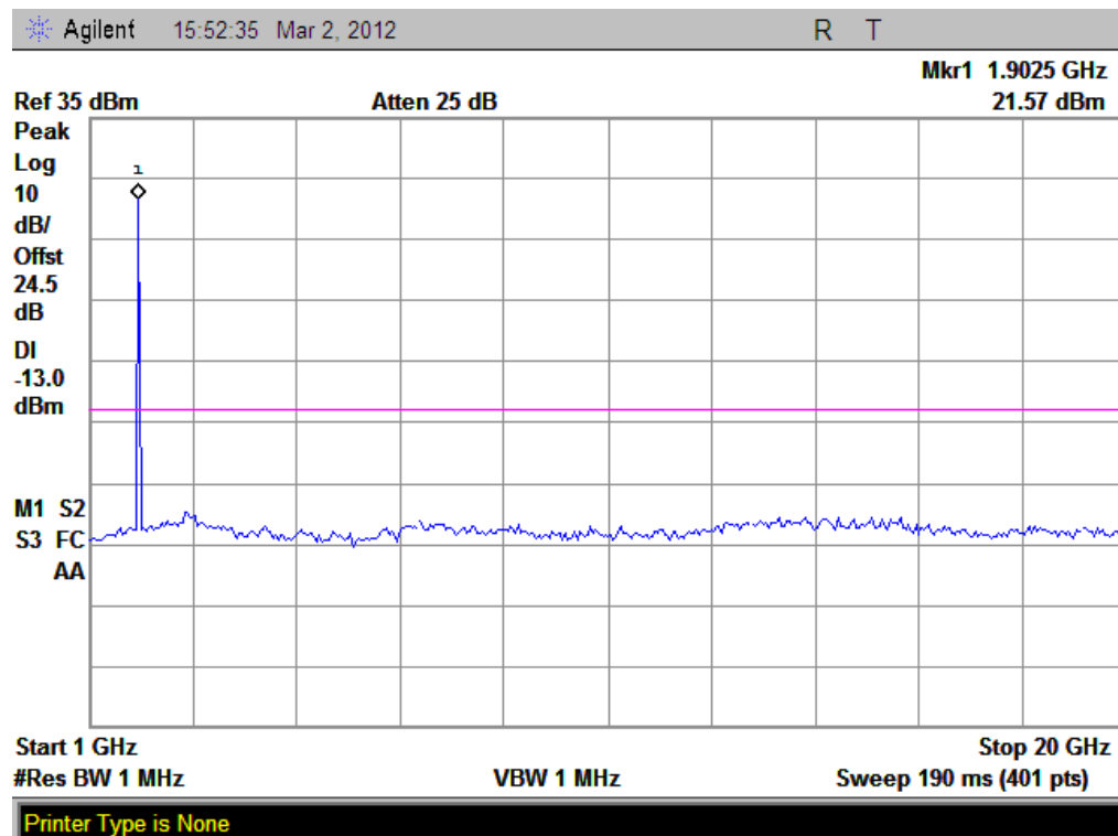
(Plot J3.1: GPRS 1900MHz Channel = 810, 1GHz to 20GHz)
