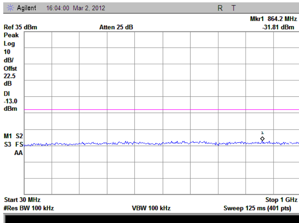
(Plot B3: EDGE 1900MHz Channel = 810, 30MHz to 1GHz)
