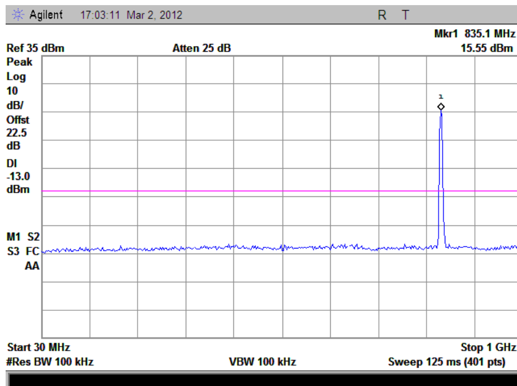
(Plot C2: WCDMA850MHz Channel = 4175, 30MHz to 1GHz)
