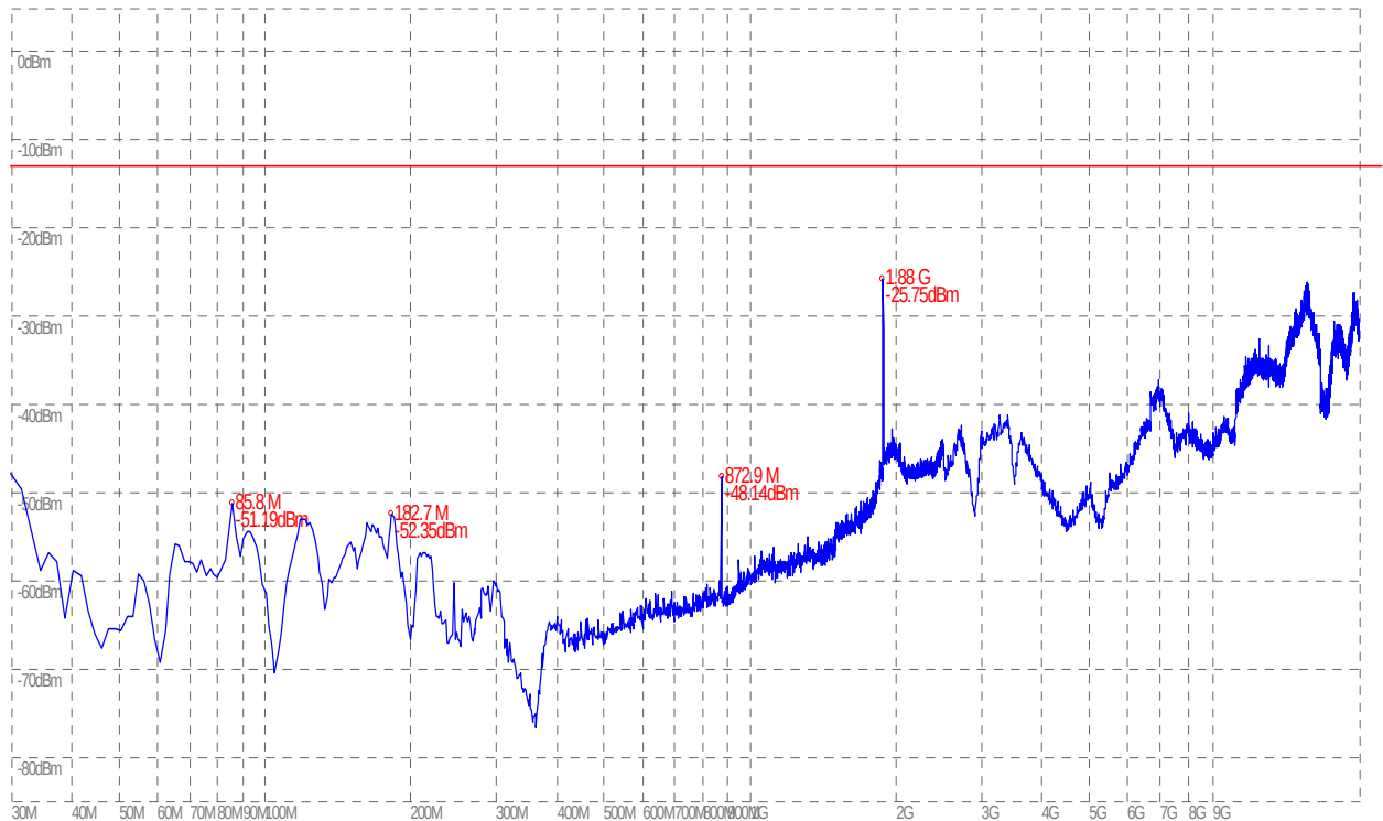
(Plot J.4: GPRS 1900MHz Channel = 661, Test Antenna Vertical)
