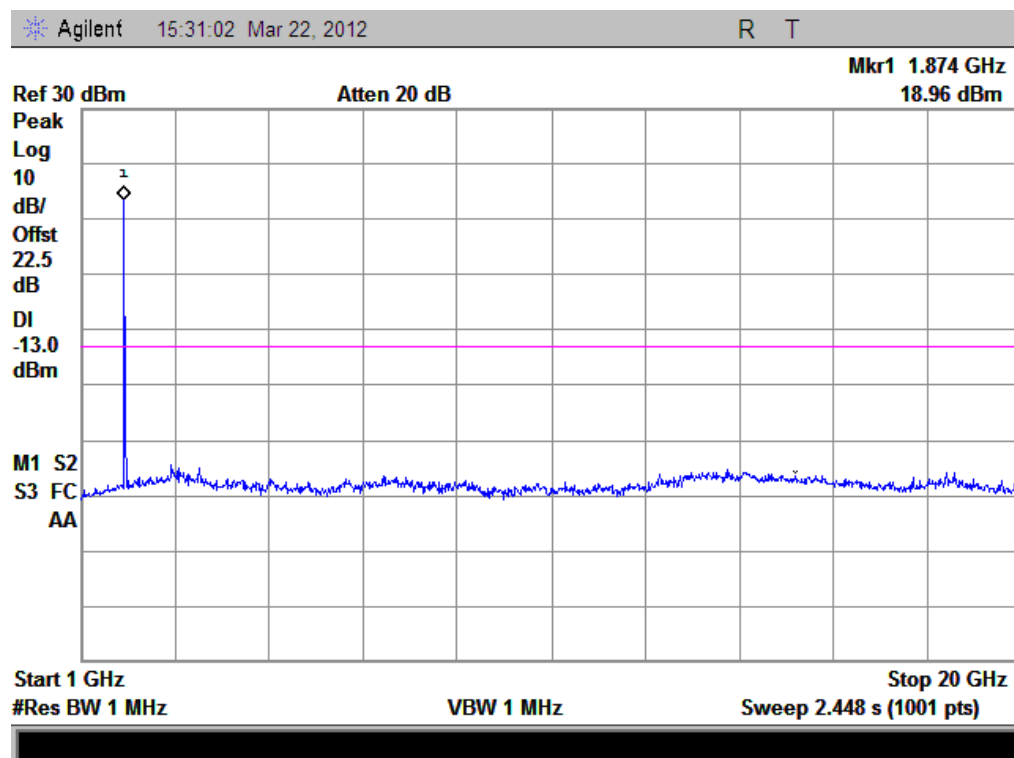
(Plot H2.1: HSUPA1900MHz Channel = 9400, 1GHz to 20GHz)
