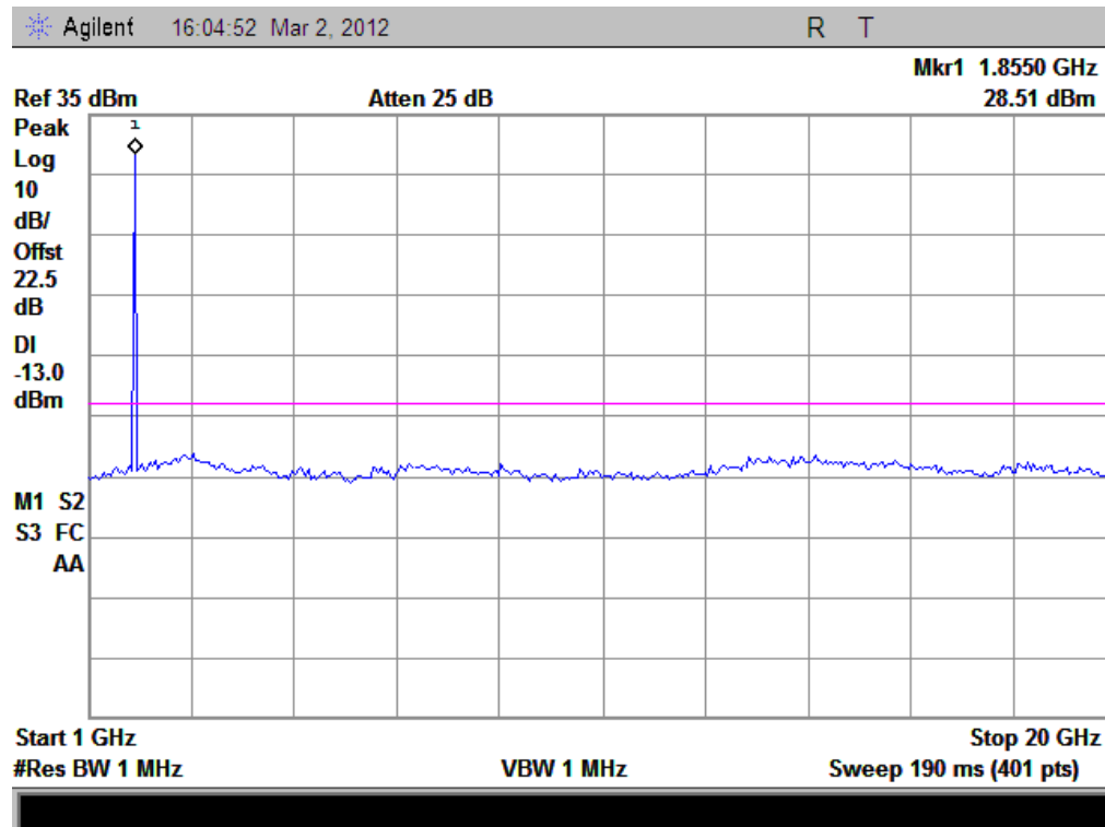
(Plot B1.1: EDGE 1900MHz Channel = 512, 1GHz to 20GHz)
