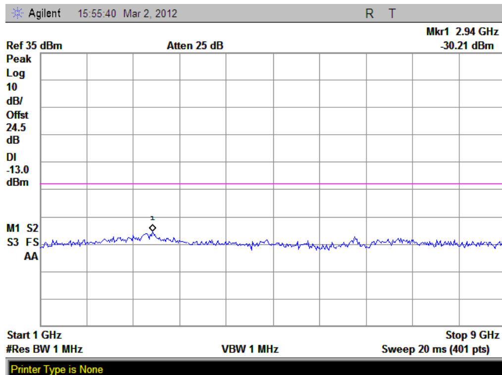
(Plot I1.1: GPRS 850MHz Channel = 128, 1GHz to 9GHz)
