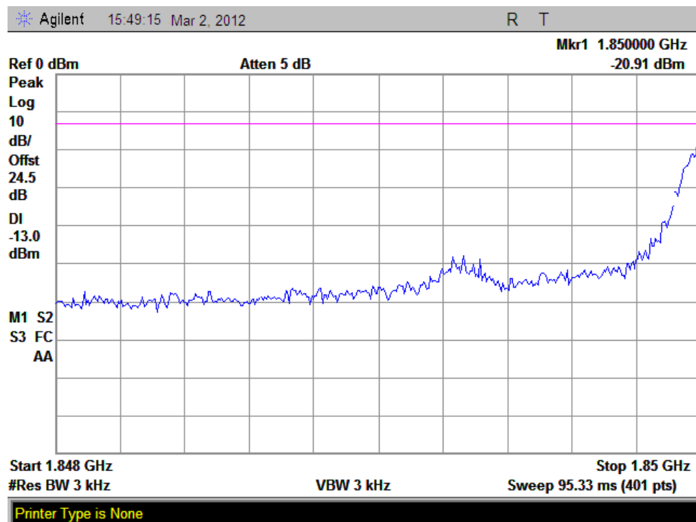
(Plot S: GPRS 1900 Channel = 512)
