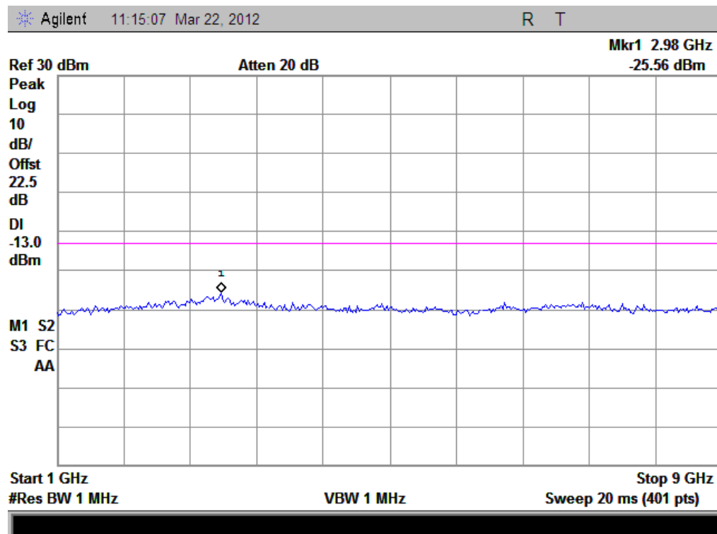
(Plot G2.1: HSUPA 850MHz Channel = 4175, 1GHz to 9GHz)
