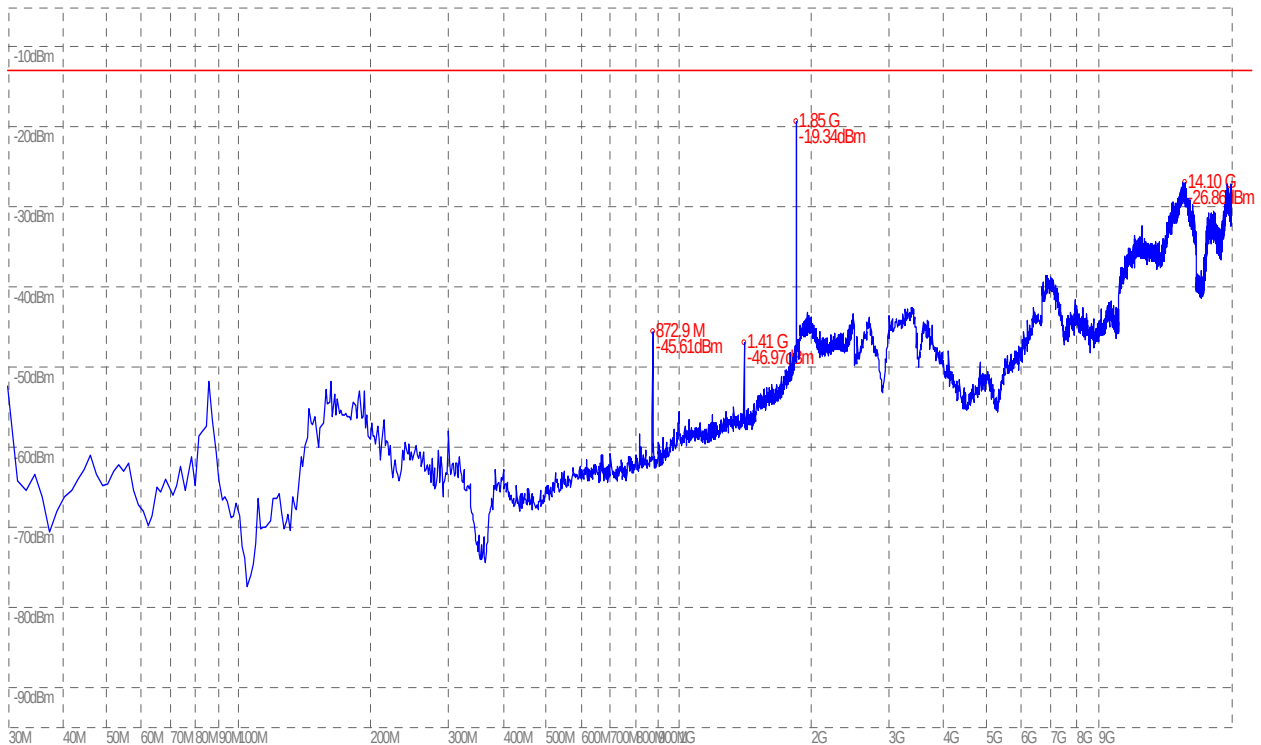
(Plot B.2: EGPRS 1900MHz Channel = 512, Test Antenna Vertical)
