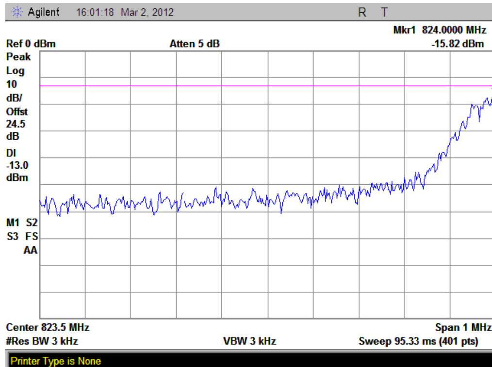
(Plot Q: GPRS 850 Channel = 128)
