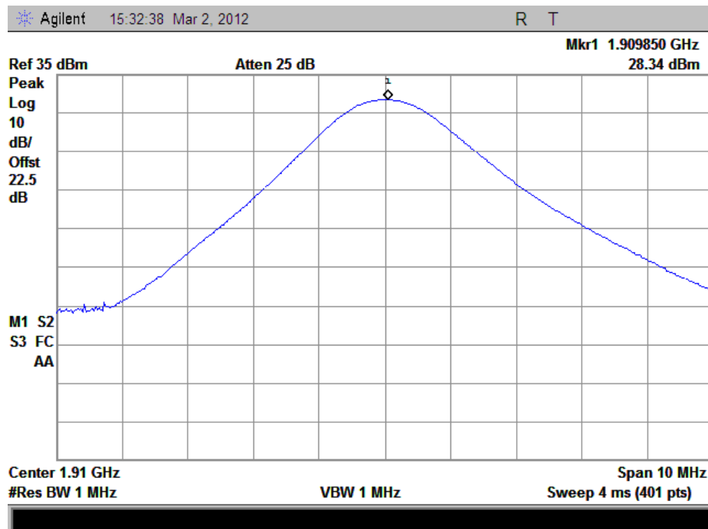
(Plot D3: EGPRS 1900Hz Channel = 810)
