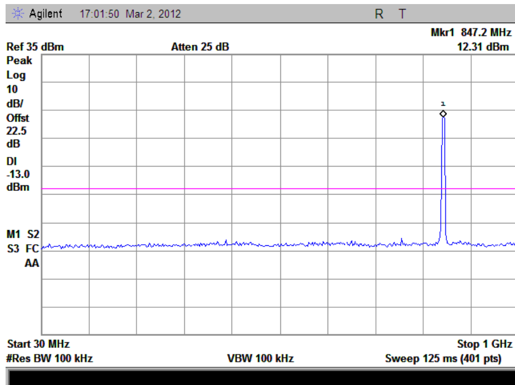
(Plot C3: WCDMA850MHz Channel = 4233, 30MHz to 1GHz)
