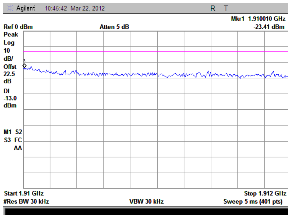
(Plot P: HSUPA 1900 Channel = 9538)
