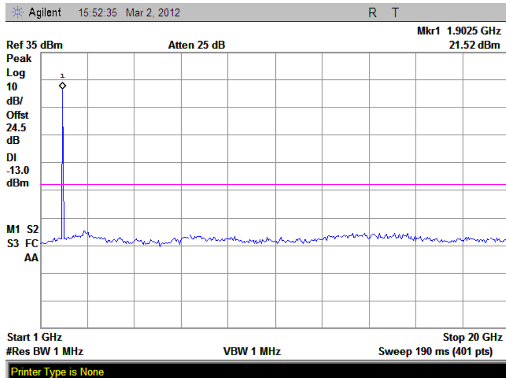
(Plot B3.1: EDGE 1900MHz Channel = 810, 1GHz to 20GHz)
