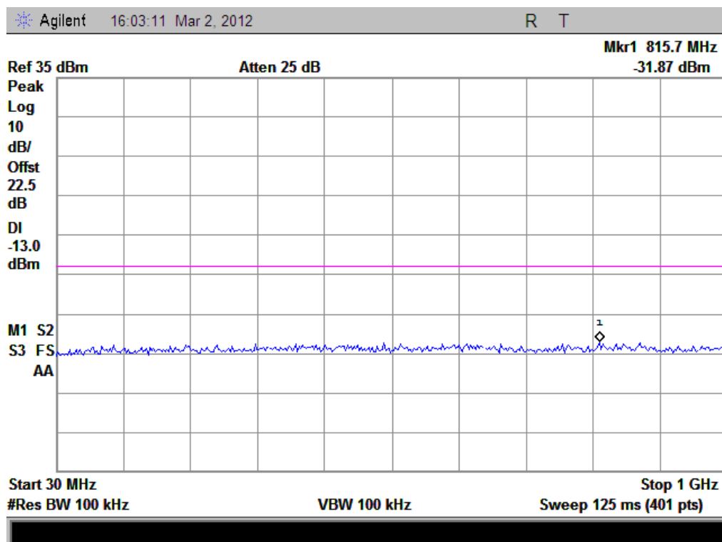
(Plot B1: EDGE 1900MHz Channel = 512, 30MHz to 1GHz)
