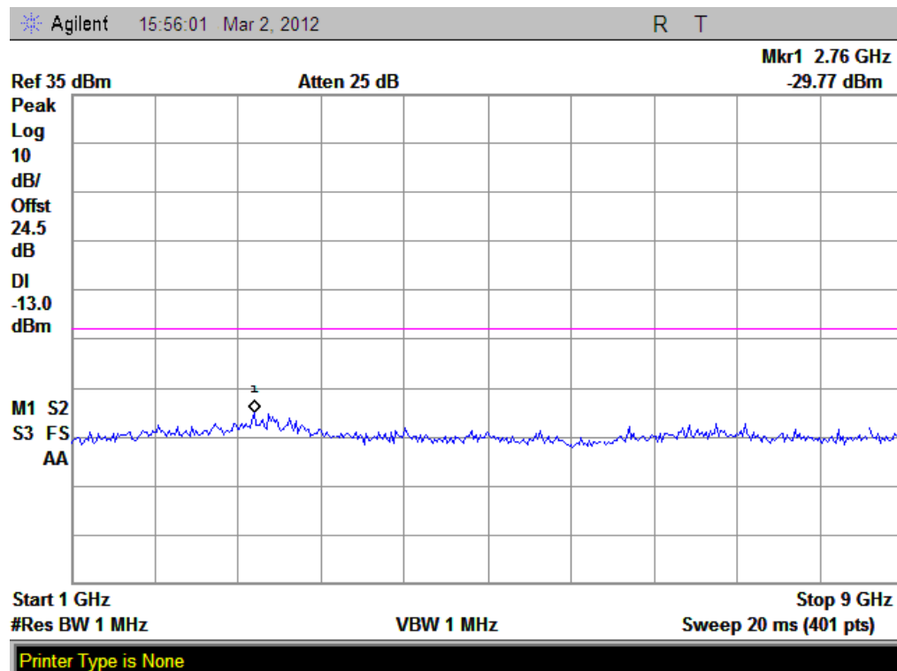
(Plot I 2.1: GPRS 850MHz Channel = 190, 1GHz to 9GHz)
