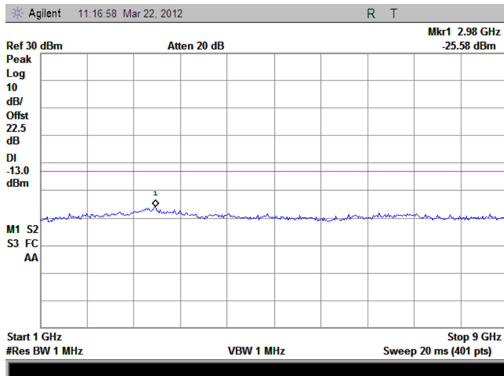
(Plot G3.1: HSUPA850MHz Channel = 4233, 1GHz to 9GHz)
