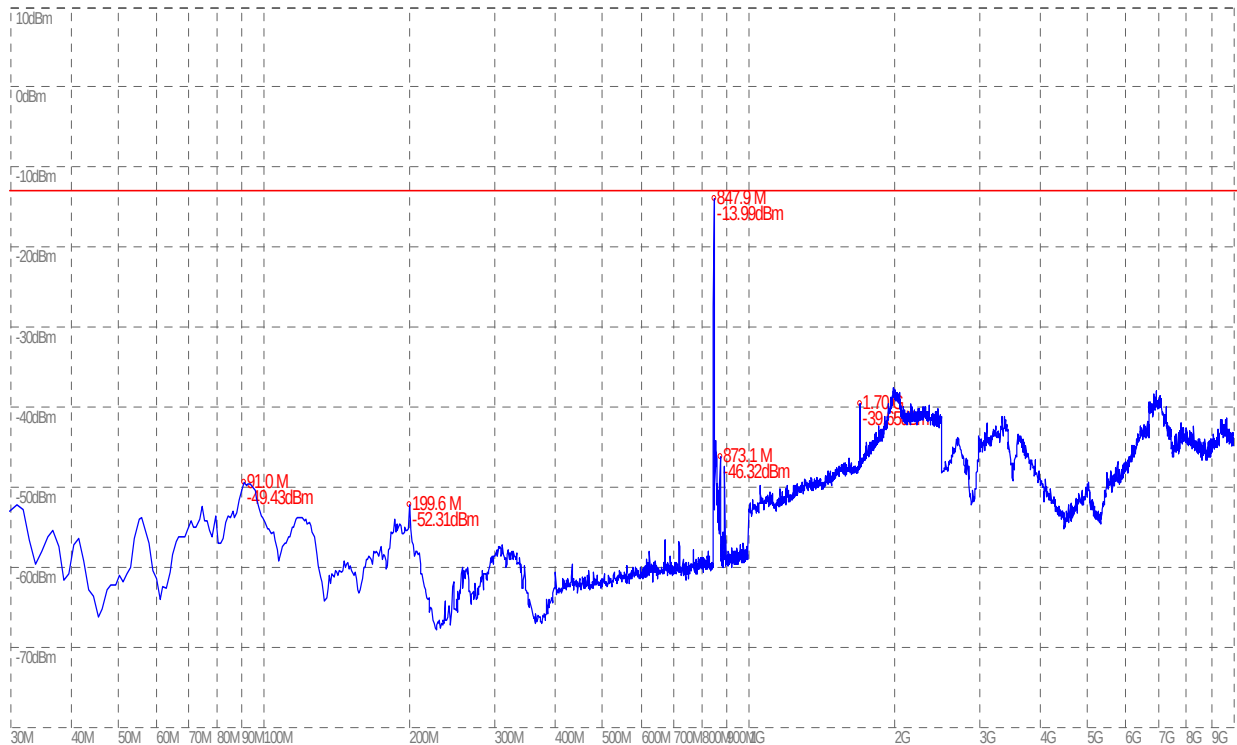
(Plot I.6: GPRS 850MHz Channel = 251, Test Antenna Vertical)
