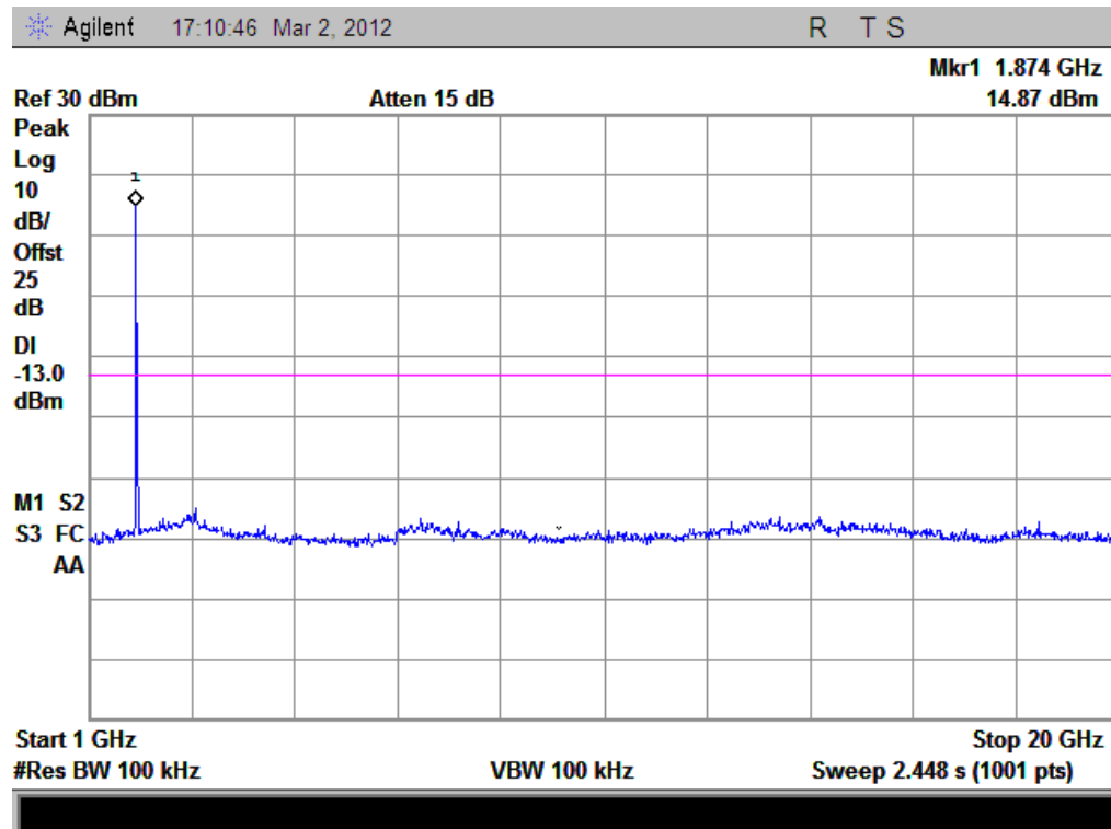
(Plot D2.1: WCDMA1900MHz Channel = 9400, 1GHz to 20GHz)
