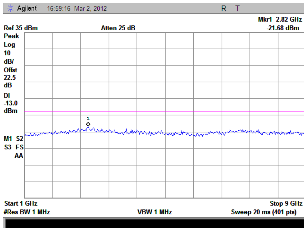
(Plot C3.1: WCDMA850MHz Channel = 4233, 1GHz to 9GHz)
