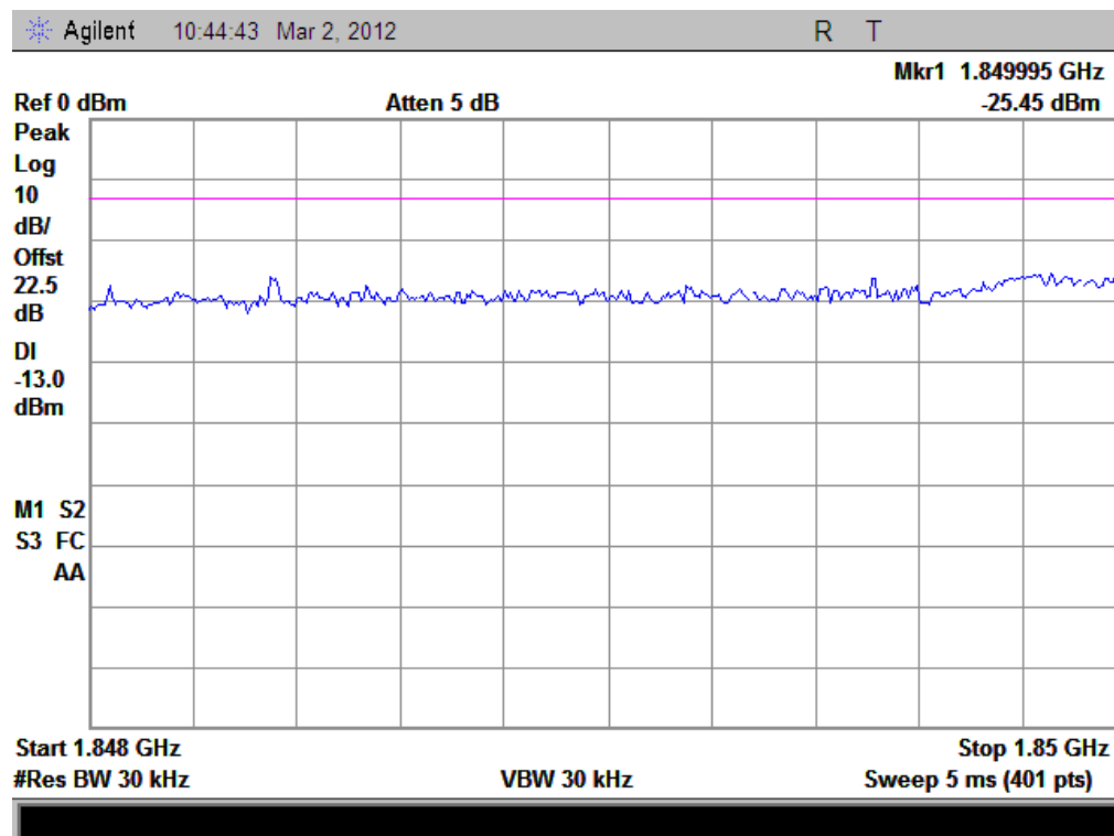
(Plot O: HSUPA 1900 Channel = 9262)
