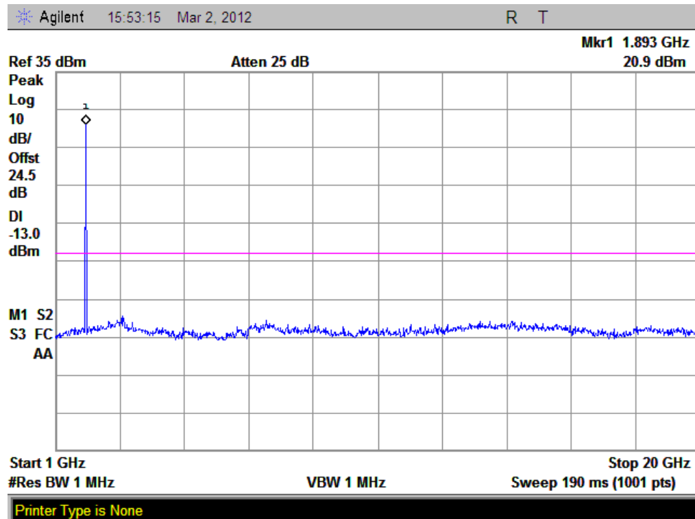
(Plot B2.1: EDGE 1900MHz Channel = 661, 1GHz to 20GHz)
