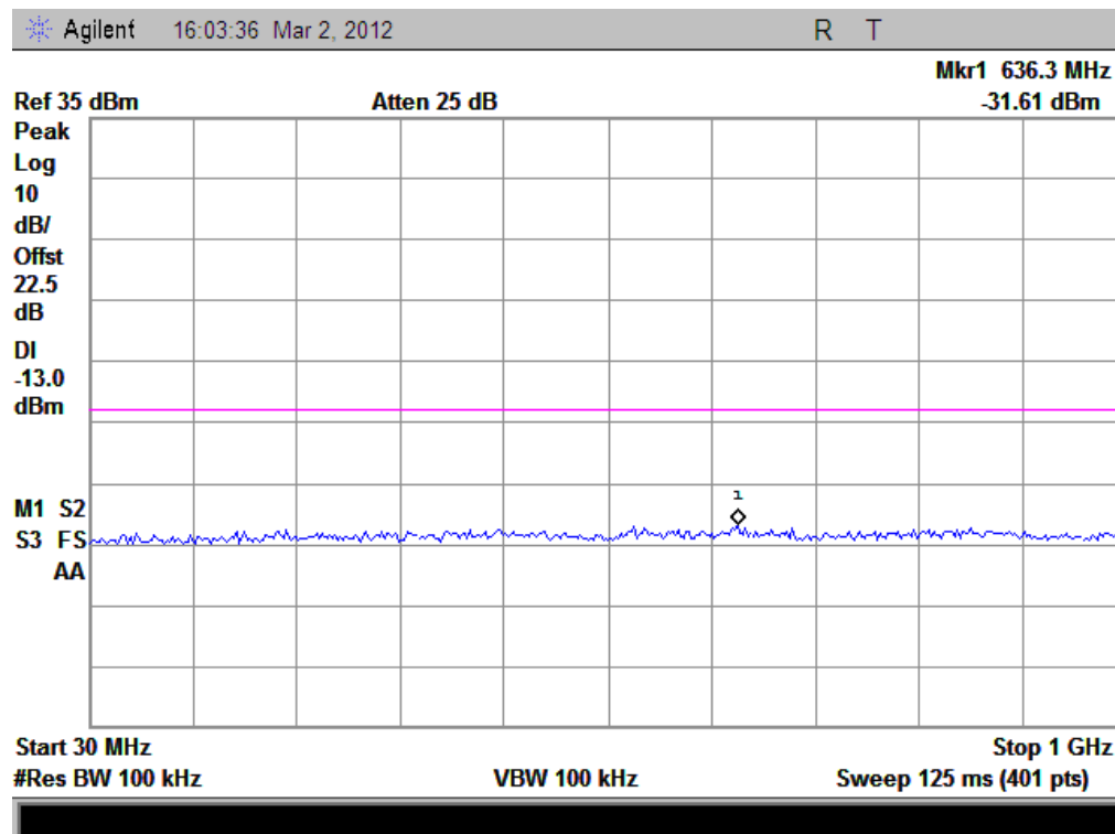
(Plot B2: EDGE 1900MHz Channel = 661, 30MHz to 1GHz)
