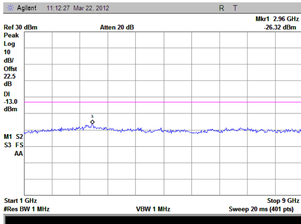
(Plot G1.1: HSUPA 850MHz Channel = 4132, 1GHz to 9GHz)
