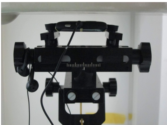
Back Face of DUT with Earphone to Phantom 1 cm Gap
