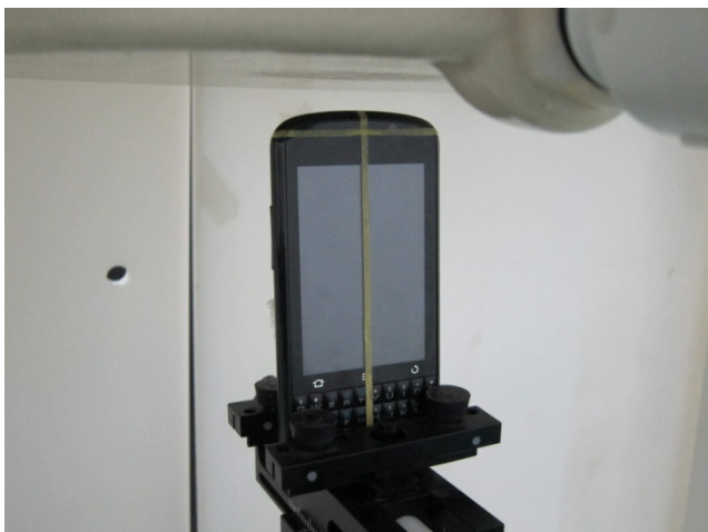
Top Side of DUT with Phantom 1 cm Gap
