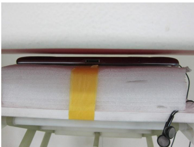
Bottom Face of EUT with earphone, 0.4 cm Gap to the Phantom
