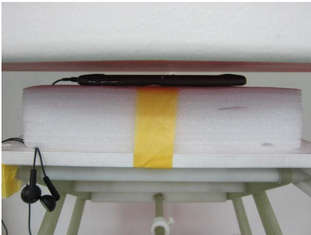
Bottom Face of the EUT with Phantom 0.9 cm Gap
