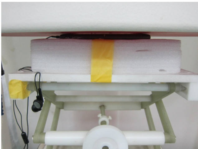
Bottom Face of the EUT with Phantom 0cm Gap
