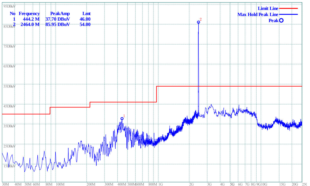
(Plot I.2: Antenna Horizontal, 30MHz to 25GHz)
