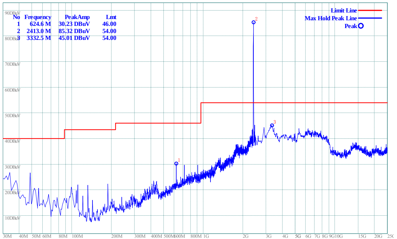
(Plot G.3: Antenna Vertical, 30MHz to 25GHz)
