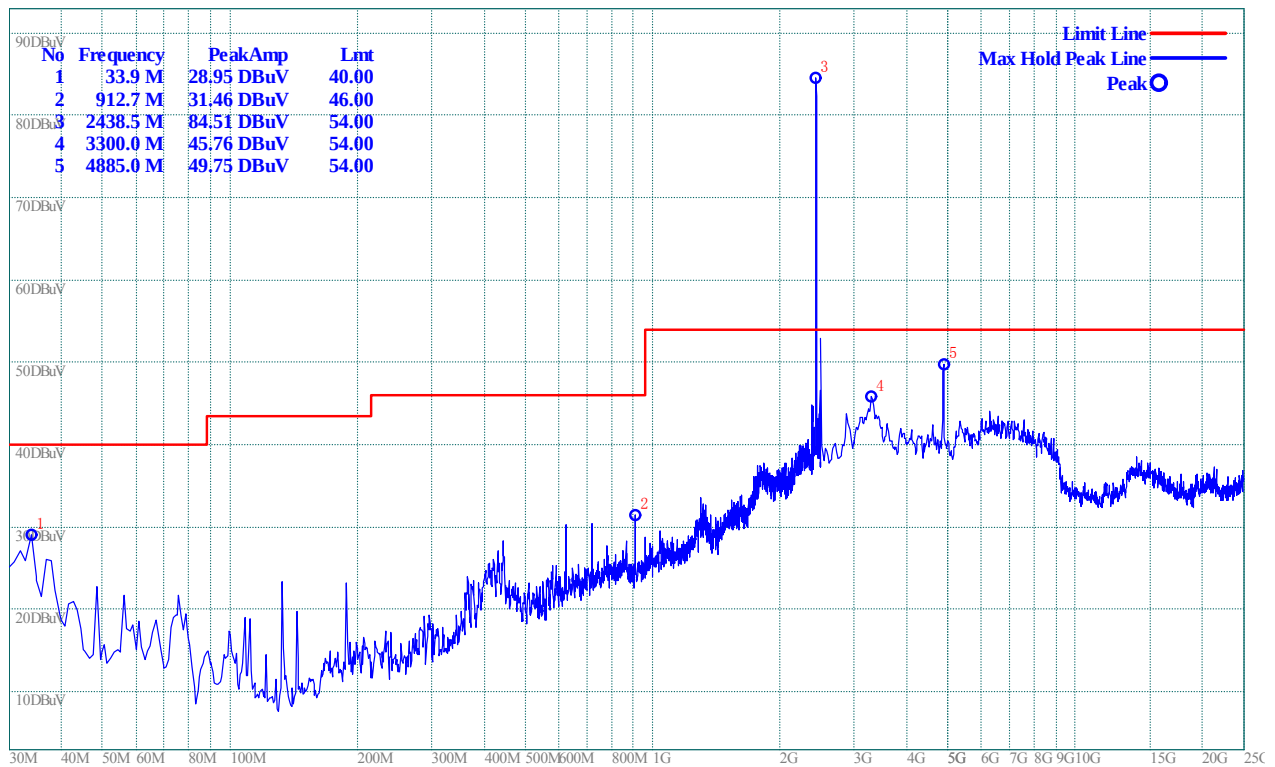
(Plot H.2: Antenna Horizontal, 30MHz to 25GHz)
