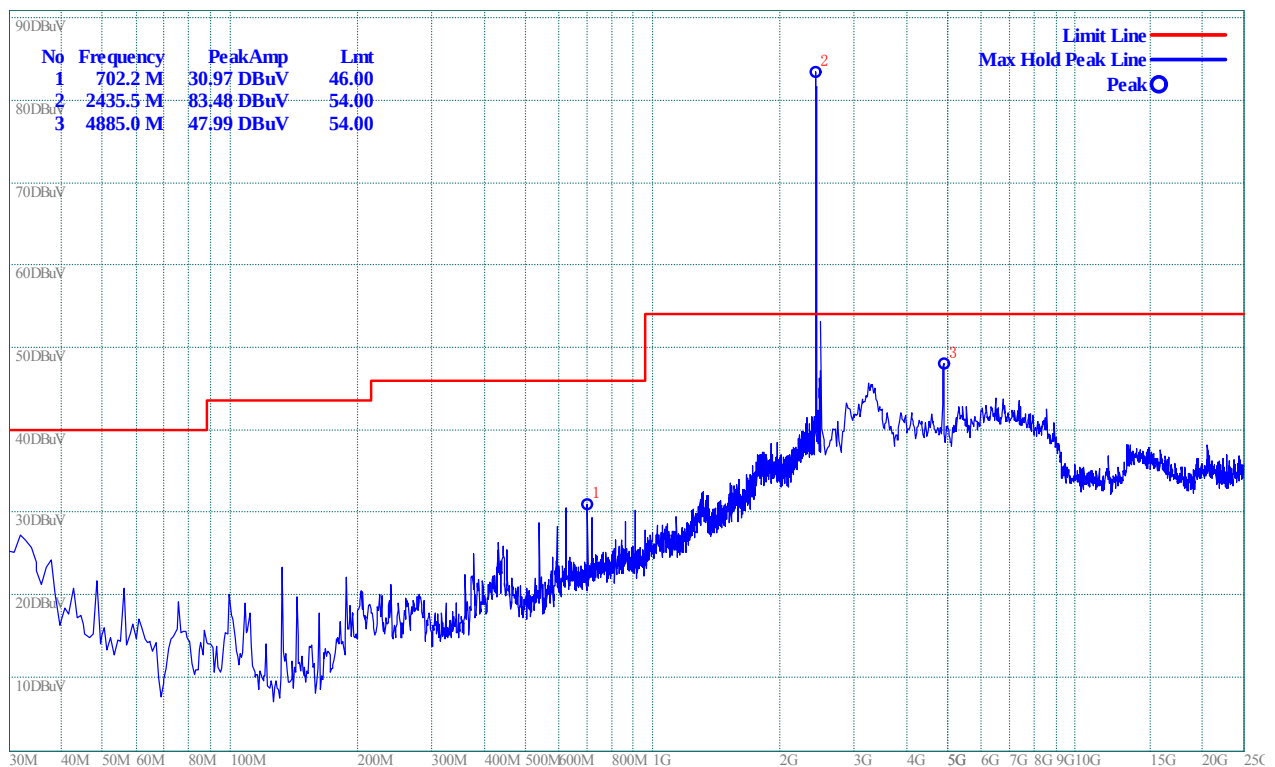
(Plot H.3: Antenna Vertical, 30MHz to 25GHz)
