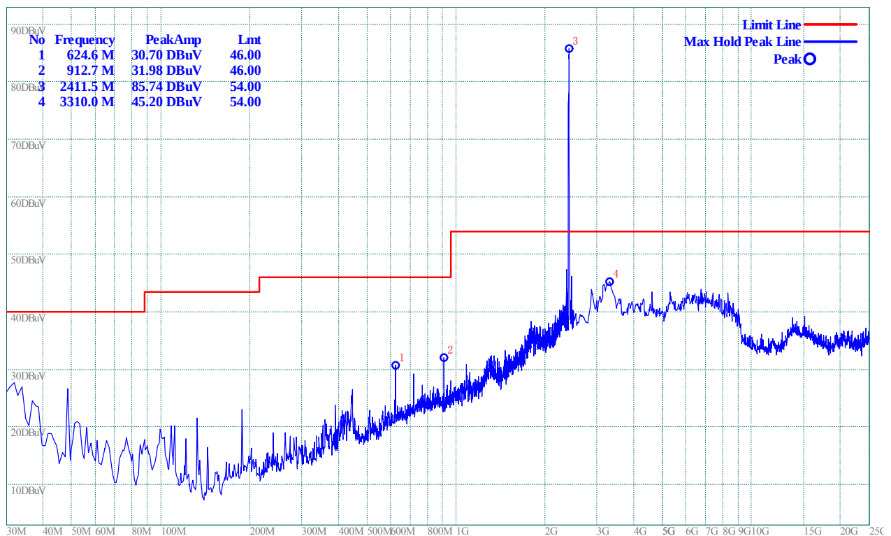
(Plot G.2: Antenna Horizontal, 30MHz to 25GHz)
