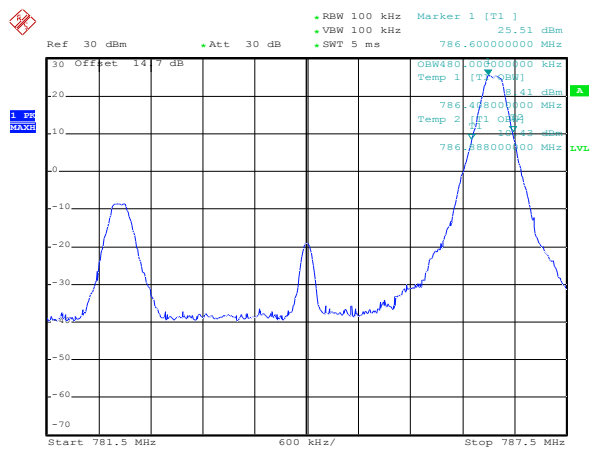
1RB Size, RB Offset 0, 16QAM
